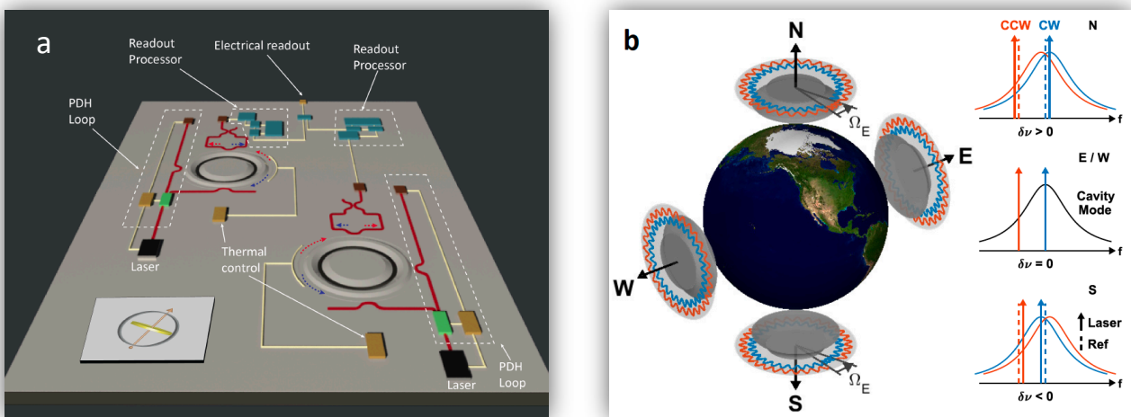
Figure 2 (adapted from ref [10]) : a, Conceptual illustration of the photonic integrated circuit using a waveguide-integrated ultra-high-Q silica resonator on a silicon chip [8]. The blue (red) arrows indicate higher (lower) Brillouin frequency. Red line: optical waveguide, Yellow line: electrical wire, Black: laser, Cyan: acousto-optic modulator, Cyan: controller, Brown: detector, Blue: electronics. b, Operation of the chip Brillouin gyroscope with its surface aligned North and South induces opposite Sagnac shifts, while with the normal axis pointed towards East and West results in no shift. Solid curve: cavity mode. Solid arrows: lasing modes with Sagnac shift. Dashed lines: lasing modes without rotation. CW: clockwise. CCW: counterclockwise.
