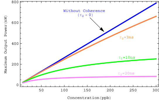
FIGURE 3. Evolution of the maximum output power (nW) versus concentration for three values of \tau_2 : 3 ns, 10 ns and 20 ns. \tau_1 was assumed to be 10 ms.
