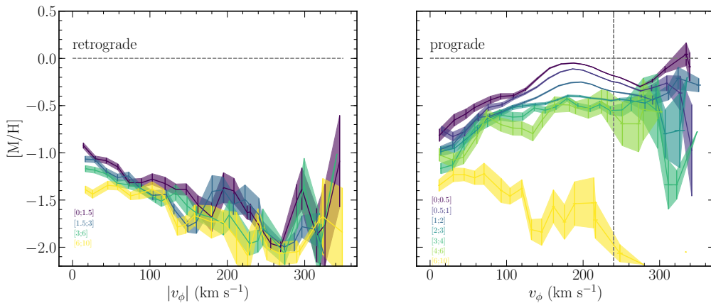
Fig. 10. Same as Fig. 8, but for the outer Galaxy ( R = [9.2-11.2] kpc).
