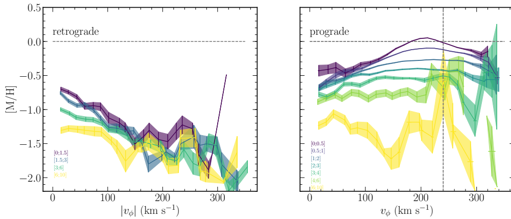
Fig. 9. Same as Fig. 8, but for the inner Galaxy ( R = [5.2-7.2] kpc).
