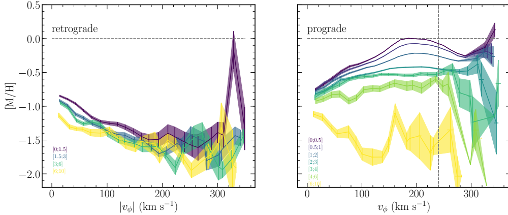
Fig. 8. v_\phi vs [M/H] for the stars in the Solar cylinder ( R = [7.2-9.2] kpc). Different colours correspond to different distances from the Galactic plane (darker colours correspond to the closest to the plane, yellow colours to the farthest distances), the range in kpc being reported at the lower-left corner of each plot. The vertical dashed line is at V_{\text{LSR}} and horizontal dashed line is at solar metallicity. Vertical error bars correspond to \sigma_{[M/H]}/\sqrt{N} , where N is the number of stars in a given bin and \sigma_{[M/H]} is the standard deviation of the metallicity inside that bin.
