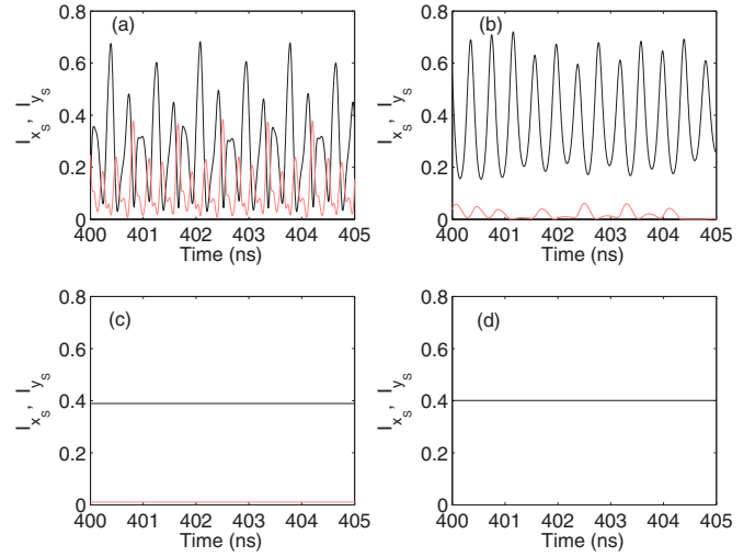
FIG. 11. (Color online) Time traces of the x -LP (black) and y -LP (red) slave laser mode intensities for different values of the spin-flip relaxation rate parameter: (a) \gamma_s=10 ns ^{-1} , (b) \gamma_s=30 ns ^{-1} , (c) \gamma_s=40 ns ^{-1} , (d) \gamma_s=300 ns ^{-1} .
