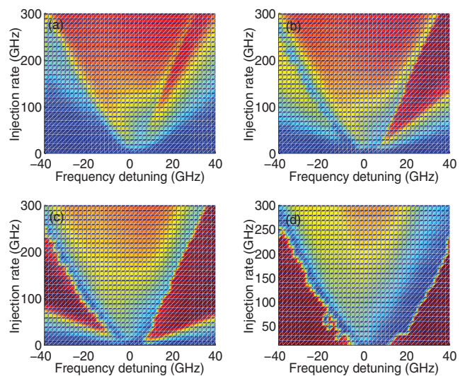
FIG. 9. (Color online) Same as Fig. 6 but with different values of the spin-flip relaxation rate parameter: (a) \gamma_s = 10 ns -1 , (b) \gamma_s = 30 ns -1 , (c) \gamma_s = 40 ns -1 , (d) \gamma_s = 300 ns -1 .
