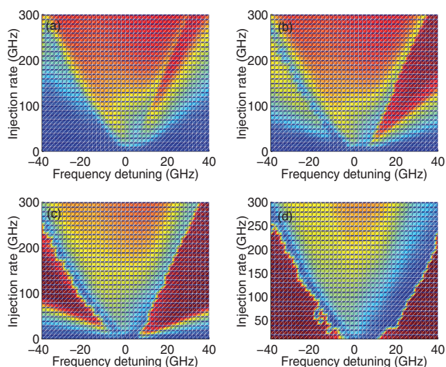
FIG. 9. (Color online) Same as Fig. 6 but with different values of the spin-flip relaxation rate parameter: (a) \gamma_s = 10 ns ^{-1} , (b) \gamma_s = 30 ns ^{-1} , (c) \gamma_s = 40 ns ^{-1} , (d) \gamma_s = 300 ns ^{-1} .
