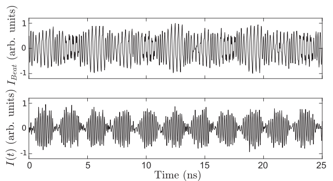
FIG. 2. Example time traces from the beat signal ( I_{\text{Beat}} ) and optical intensity [ I(t) ] measurements simultaneously acquired from the two photodiodes.
