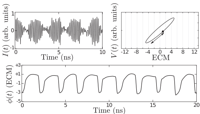
FIG. 4. The first instability, \beta , gives rise to a quasiperiodic-like trajectory in I(t) with two distinct frequencies seen in the dynamics. The CW emission in I(t) is around ECM +1, but the fast oscillation portion of I(t) coincides with movement in the optical phase towards the MGM (negative ECMs). As feedback is increased the optical phase moves further and further in phase space towards negative modes (MGM) as the ellipse gets larger (not shown).
