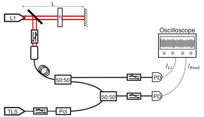
FIG. 1. Schematic diagram of the laser subjected external optical feedback and heterodyne measurement. The MQW laser under study (L1) is subjected to optical feedback from a mirror with a reflectivity of 99.97%. The feedback ( \eta ) is controlled by rotating a quarter-wave plate relative to a fixed linear polarizer. TLS is the tunable laser source for heterodyning. PD, Pol, and 50:50 stand for photodiode, polarization controller, and fiber-optic splitter or combiner, respectively.
