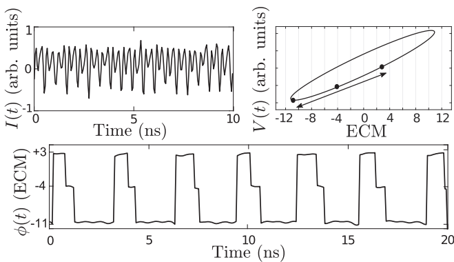
FIG. 7. Frequency halving of the final LC frequency is observed as a period-doubled trajectory, \epsilon , in I(t) . The optical phase covers a large portion of phase space (ECMs +3 , -4 , -11 ).
