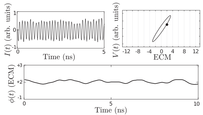
FIG. 5. An example of a limit cycle trajectory, during \gamma . We see a sinusoidal oscillation in the optical intensity. The optical frequency is centered around ECM +2.
