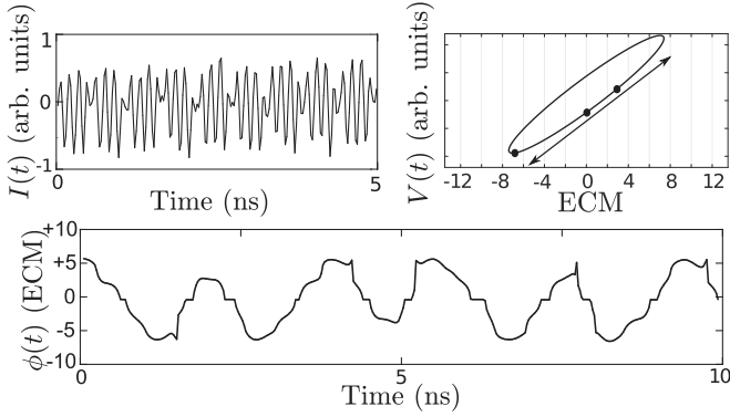
FIG. 6. An example subharmonic trajectory, during \delta , with two periodic oscillations for every one PD oscillation. From the optical phase, we see periodic oscillations around m > 0 ECMs and PD oscillations between ECMs 0 and -7 .
