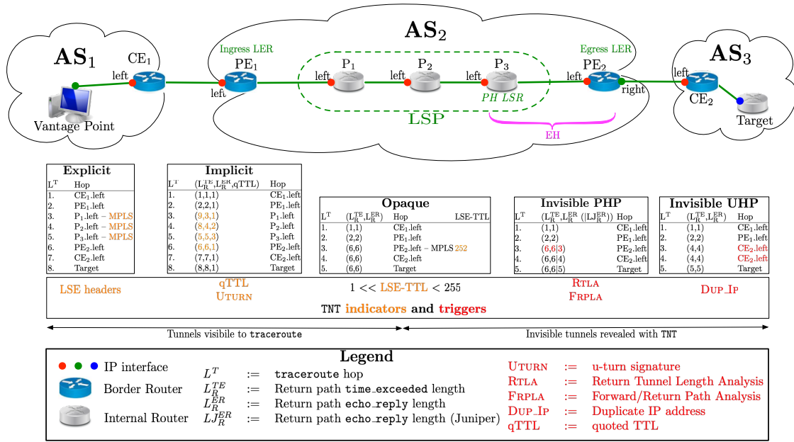
Fig. 2: Illustration of MPLS vocabulary and relationship between MPLS and traceroute. The figure is made of three parts. The upper part represents the network topology used throughout the paper to illustrate MPLS and TNT concepts. In particular, with respect to MPLS, P 1 is the LSP First Hop (FH), while P 3 is the Penultimate Hop LSR (PH LSR). In case of PHP, P 3 is the Ending Hop (EH) responsible for removing the LSE, while, with UHP, it is the Egress LER (PE 2 ). The middle part of the figure presents our MPLS classification. Finally, the bottom part of the figure provides triggers and indicators of an MPLS tunnel presence when probing with TNT. The relationship between the trigger/indicator and the observation made with probing is provided in red. Additional information (e.g. time-exceeded path length) are provided to illustrate TNT in Sec. V.
