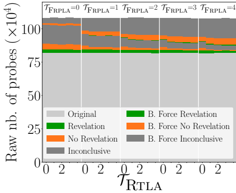
Fig. 4: Probing cost associated to TNT according to \mathcal{T}_{FRPLA} and \mathcal{T}_{RTLA} thresholds. Here we also evaluate their uses with a value of 0 leading to 25 combination pairs (instead of 16 previously). The X-Axis plots, for multiple \mathcal{T}_{FRPLA} (see labels above) the corresponding \mathcal{T}_{RTLA} \in [0, 4] .
