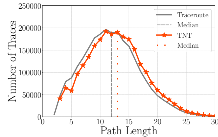
Fig. 8: Path length distribution correction with TNT. “Median” corresponds to the median path length for classic traceroute exploration (dashed grey) and when additional paths are revealed through TNT (dotted red).
