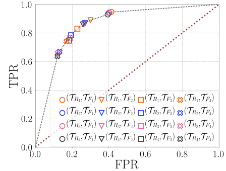
Fig. 3: Receiver operating characteristic (ROC) curve providing the performances of TNT according to the thresholds used for revealing Invisible tunnels. \mathcal{T}_{R_x} refers to \mathcal{T}_{RTLA} with the value x , while \mathcal{T}_{F_y} to \mathcal{T}_{FRPLA} with the value y .
