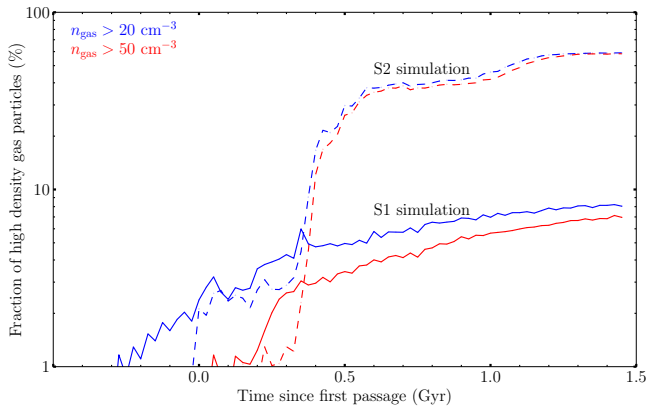
Figure 12. Temporal variation of the fraction of gas particles with relatively high local number densities n_{\text{gas}} in the S1 (solid curves) and S2 (dashed curves) simulations, respectively. n_{\text{gas}} is calculated as the average within cubic cells with 50 pc side lengths. Two different n_{\text{gas}} thresholds (in the regime of cold neutral medium phase) are used to illustrate the temporal variation.
