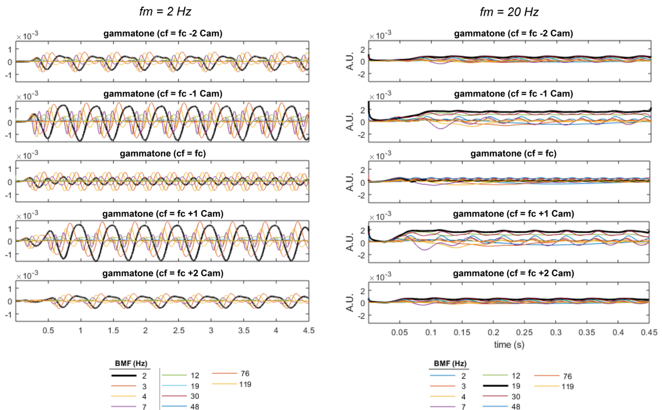
FIG. 4. (Color online) Internal representation of a 2-Hz (left panels) or 20-Hz (right panels) FM signal (500-Hz carrier) for each channel [with center frequency (cf)] and each modulation filter [with best modulation frequency (BMF)]. The black line indicates the output of the modulation filter closest to the target rate (2 or 19 Hz).
