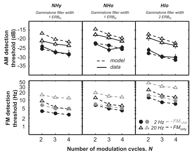
FIG. 6. As Fig. 5, but with the widths of the gammatone filters set to 1 \text{ERB}_N for the NHy and NHo models, and 2 \text{ERB}_N for the HIo model.
