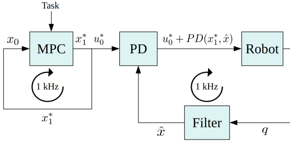
Fig. 2: Open-loop MPC: replan based on predictions. This control scheme is representative of MPC controllers found in the literature such as in [25].
