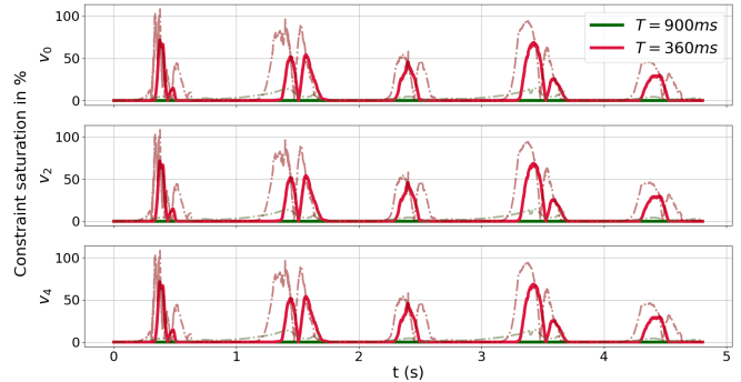
(b) Joint velocities saturation (desired in thin dashed line)
