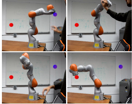
Fig. 1: Pick-and-place task, with high dynamics and precision thanks to our state-feedback MPC, but keeping high compliance thanks to the low-level torque control.
