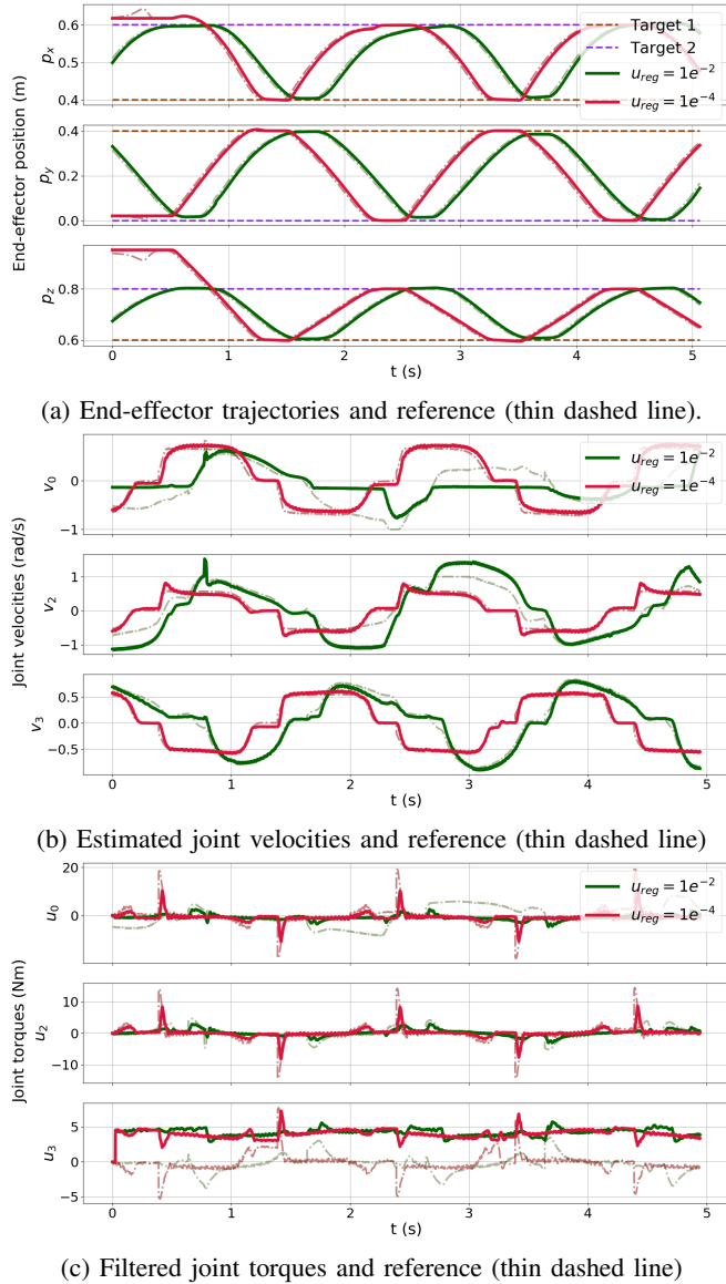
Fig. 9: When the control regularization term decreases, the trajectories are less relevant: the velocity tends toward a square signal and the torque exhibits sharp peaks
