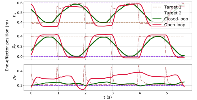
(a) End-effector trajectories (desired in thin dashed line).
