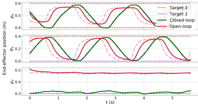
Fig. 6: Reducing the cost weights by setting \alpha = 20 , \beta = 0.8 , the open-loop MPC (red) results in a smaller tracking error (average norm 0.7 vs 1.6 in Figure 5) but a loss in the end-effector precision, as seen by comparison with the original closed-loop MPC trajectory (green) duplicated from Figure 5.
