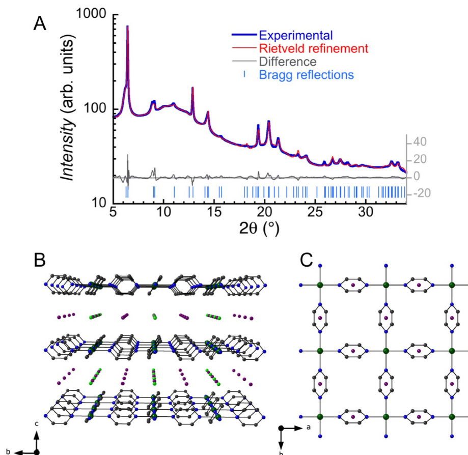
Fig. 3. Structural model of \text{Li}_{0.7}[\text{Cr}(\text{pyz})_2]\text{Cl}_{0.7}\cdot 0.25(\text{THF}) ( 2·0.25(THF) ). (A) The best Rietveld refinement (red trace; R_1 = 4.23 \% ) of the synchrotron PXRD pattern of 2·0.25(THF) at 290 K (after cooling from 500 K in a sealed capillary; blue trace) is shown together with the experimental/model difference (grey trace) and calculated Bragg reflections (blue bars). (B) Perspective view (along the a direction) of 2·0.25(THF) showing the alternation of \{\text{Li}_{0.7}\text{Cl}_{0.7}\} and neutral \text{Cr}^{\text{II}}(\text{pyz})_2 layers stacking along the c direction. (C) Eclipsed layered structure viewed along the c direction. Cr: dark green, N: blue, C: black. Cl (light green) and Li (purple) are shown at a fixed occupancy of 70% according to the elemental composition. Hydrogen atoms have been omitted for clarity.
