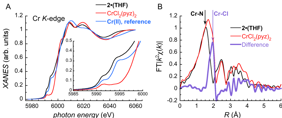
Fig. 2. XANES and EXAFS spectra at the Cr K -edge at 295 K. (A) Normalized XANES spectra of 2 ·(THF) (black trace), \text{CrCl}_2(\text{pyz})_2 (red trace) and Cr(II) reference (blue trace). Inset: magnified view of the near-edge region. (B) Fourier-transform (FT) EXAFS spectra for 2 ·(THF) (black trace) and \text{CrCl}_2(\text{pyz})_2 (red trace; see Figs. S9–S10 for additional EXAFS data, 28). The difference of the two data sets is shown in purple.
