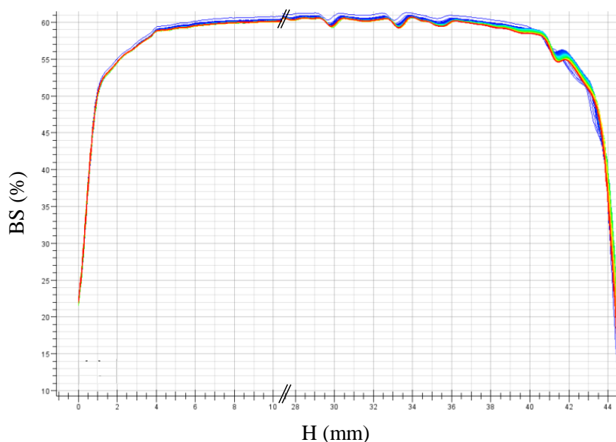
Figure 9. Turbiscan® measurements of ODA-SBR#01 latex.
