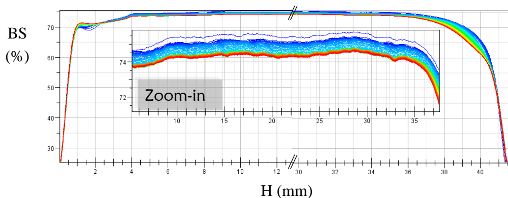
Figure 8. Turbiscan® measurements of the HD-SBR#01 latex.
