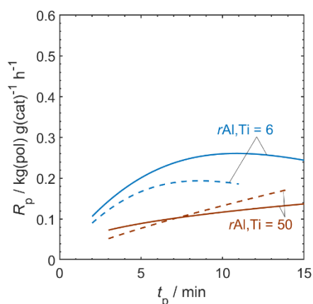
Figure 3. Effects of H_2 and dosage of TEA on kinetics. (Solid lines) with H_2 , (dashed lines) without H_2 . P_{C_2} = 4 bar, P_{C_4} = 2 bar, P_{H_2} = 0.76 bar (if applicable).
