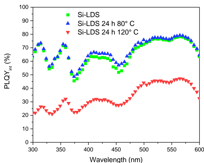
Figure 10. Variations in PL QY_{int} as a function of the excitation wavelength for Si-LDS film and Si-LDS films heat-treated at 80 °C and 120°C for 24 hours.
