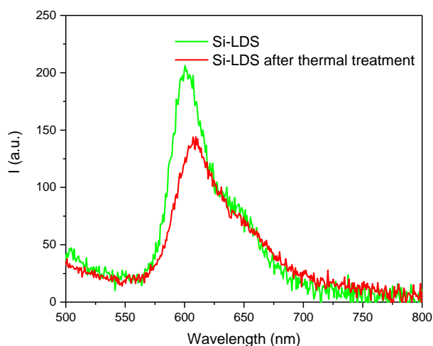
Figure 11. Emission spectra of Si-LDS films before and after thermal treatment for 24h at 120°C ( \lambda_{exc} = 480 nm).
