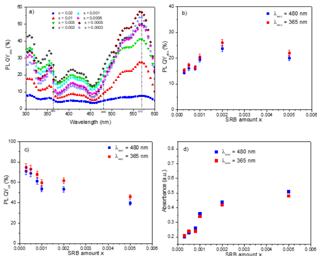
Figure 3. (a) Variation in PL QY abs as a function of the excitation wavelength for LDH-DS-SRB samples and variation in PL QY abs (b), internal photoluminescence quantum yield PL QY int (c) and Absorbance (d) as a function of the SRB content ( x ) for \lambda_{exc} = 480 nm and \lambda_{exc} = 365 nm.
