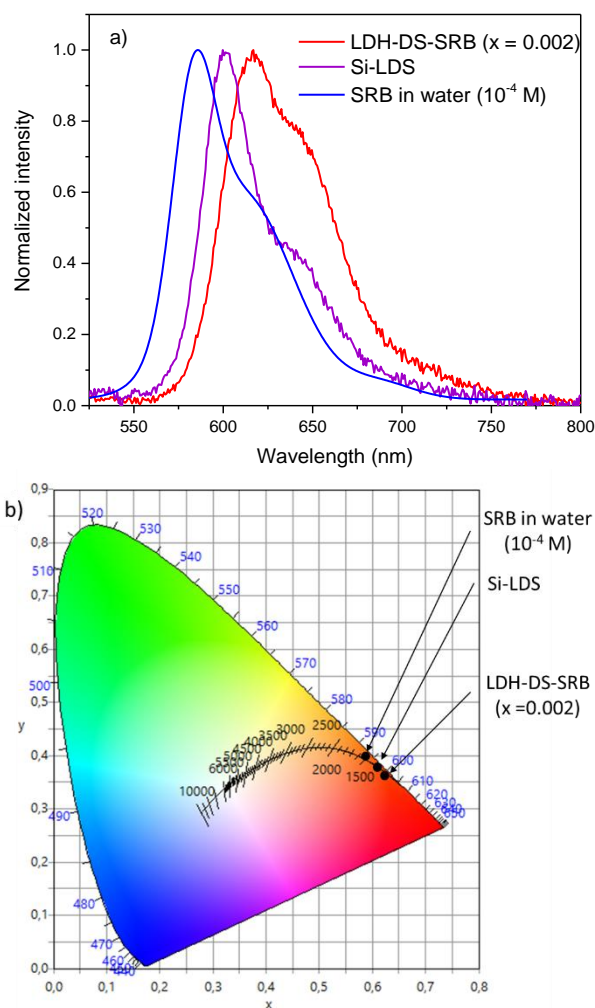
Figure 6. a) Emission spectra of the LDH-DS-SRB powder ( x=0.002 ) (red line), SRB in water solution ( 10^{-4} M) (blue line) and the silicone Si-LDS film (purple line); b) CIE chromaticity coordinates of LDH-DS-SRB powder ( x=0.002 ), SRB in water ( 10^{-4} M) and Si-LDS composite film
