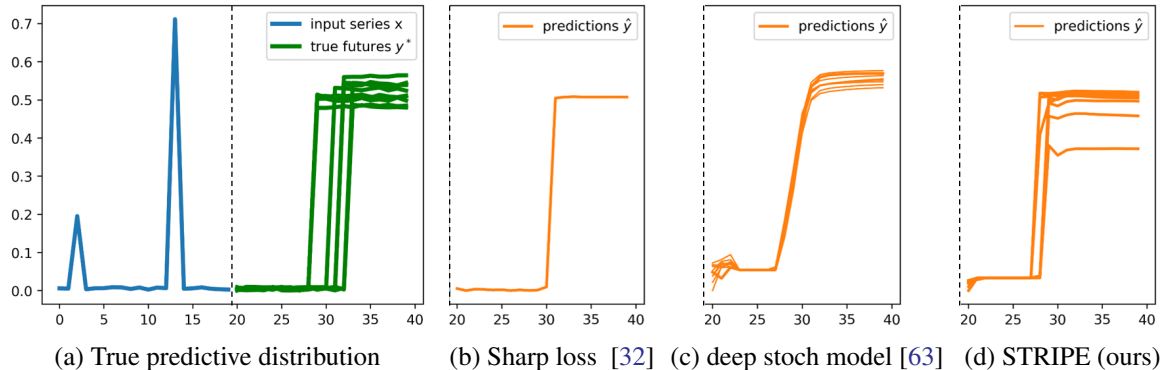
Figure 1: We address the probabilistic time series forecasting problem. (a) Recent deep learning models include a specific loss enabling sharp predictions [11, 46, 32, 56] (b), but are inadequate for producing diverse forecasts. On the other hand, probabilistic forecasting approaches based on generative models [63, 45] loose the ability to generate sharp forecasts (c). The proposed STRIPE model (d) produces both sharp and diverse future forecasts.
