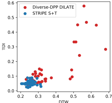
Figure 6: Scatterplot of 50 predictions in the plane (DTW, TDI), comparing STRIPE S+T v.s. Diverse DPP DILATE [63].
