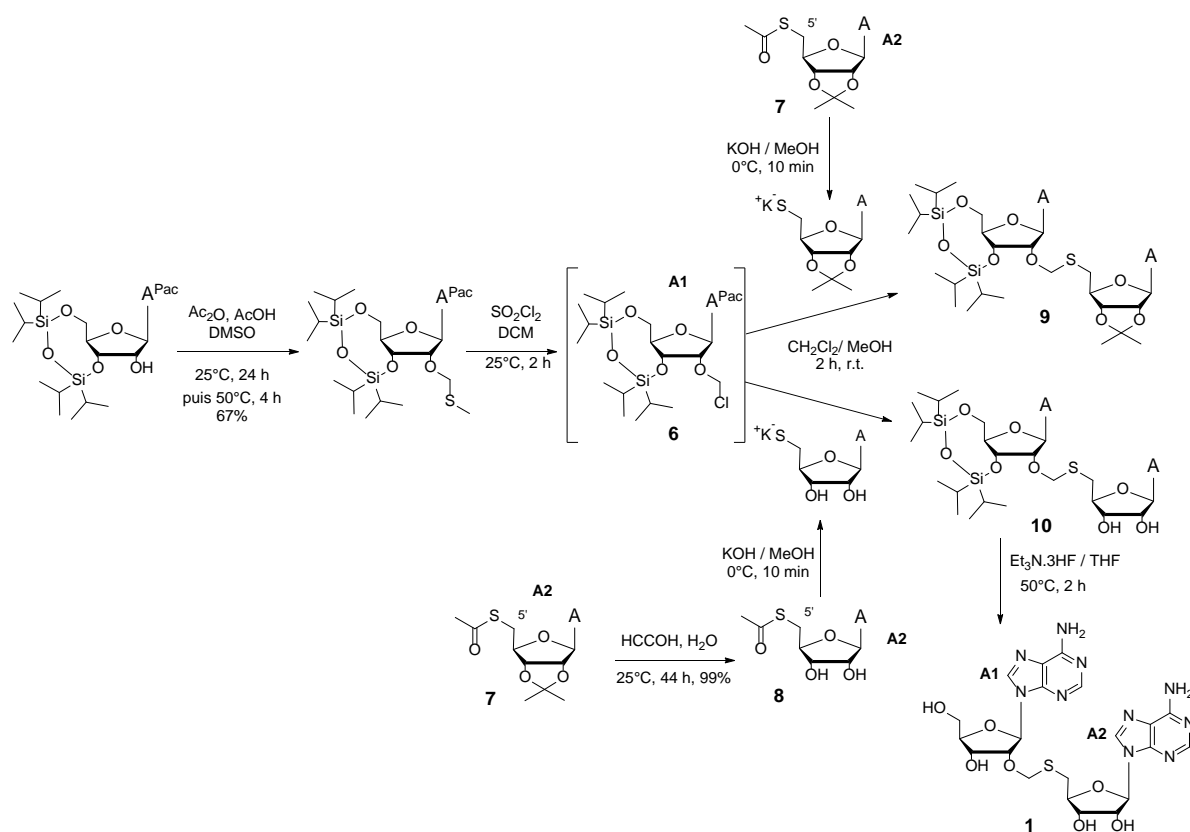
Scheme 2. Synthesis of S -(2'- O -methyladenosyl) 5'-thioadenosine 1 . A = adenine. A Pac = N 6 -phenoxycetyl adenine
