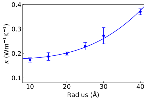
Figure 4: Thermal conductivity of FNPs computed with EMD at 300K, the error bar corresponds to the standard deviation between the 5 to 10 independent runs. The blue line is a fit to a cubic scaling law as a guide to the eye.
