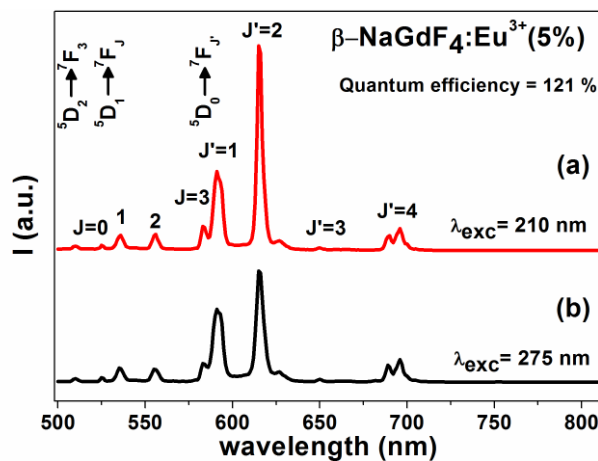
Figure 18 :Emission spectra of \beta\text{-NaGdF}_4\text{:Eu}^{3+} (5 mol%) recorded at RT upon (a)close to \text{Gd}^{3+}\text{-}{}^8\text{S}_{7/2}\rightarrow{}^6\text{G}_j excitation at 210 nm and upon (b) \text{Gd}^{3+}\text{-}{}^8\text{S}_{7/2}\rightarrow{}^6\text{I}_{7/2} excitation at 275 nm. Both spectra are scaled on the {}^5\text{D}_1\rightarrow{}^7\text{F}_j emission intensity.
