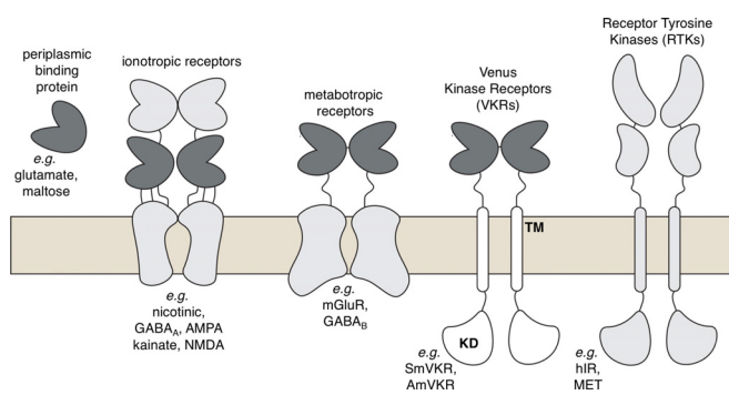
Figure 1. Proteins with Venus-flytrap-like or clamshell ligand-binding domains (LBDs). Presumably originating from periplasmic binding proteins, the Venus-flytrap domain (dark grey) has been found in all classes of transmembrane proteins, such as ion channels, GPCRs, and receptor-linked enzymes like tyrosine kinase, but VKRs are only found in invertebrates. Vertebrate RTKs do not bear clamshell LBDs.
