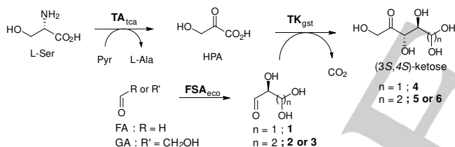
Scheme 2. One-pot cascade reaction for the synthesis of ketoses 4–6 by TK gst with convergent in situ generation of HPA using TA ica and aldehydes 1–3 using FSA eco .
