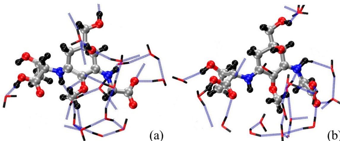
Figure 9: Evolution of the hydrogen bond network around the porphyrin-334 molecule solvated in water for the configuration 2 structure. Panel (a) shows the hydrogen bonding of the solute with solvating water at the beginning of the simulation, whereas panel (b) shows the dynamical evolution at the end of the run where the equilibrium is attained. Red, blue, gray, and black balls and sticks indicate oxygen, nitrogen, carbon, and hydrogen, respectively, while hydrogen bonds are shown as dashed blue lines.
