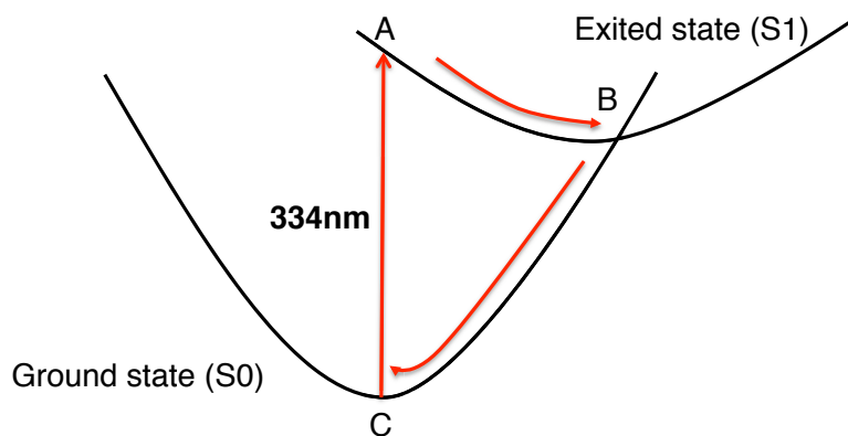
Figure 2: Schematic picture of the ground ( S_0 ) and excited ( S_1 ) states of the porphyrin-334 molecule. The transition from C to A indicates the initial vertical transition from the ground to the excited state. The transition from A to B indicates the structural relaxation at the excited state. At the point B, the system reverts to the ground state via a nonradiative transition. The transition from B to C indicates the structural relaxation at the ground state. At the point C, the porphyrin-334 acquires an excess of kinetic energy as a response to the adsorption of photons of wavelength of 334 nm. Our dynamical simulations describe the process occurring for the transition from B to C and the subsequent relaxation in the range around point C on the ground state.
