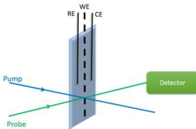
Figure 17. Electrochemical cell for transient absorption spectroelectrochemistry measurements.
