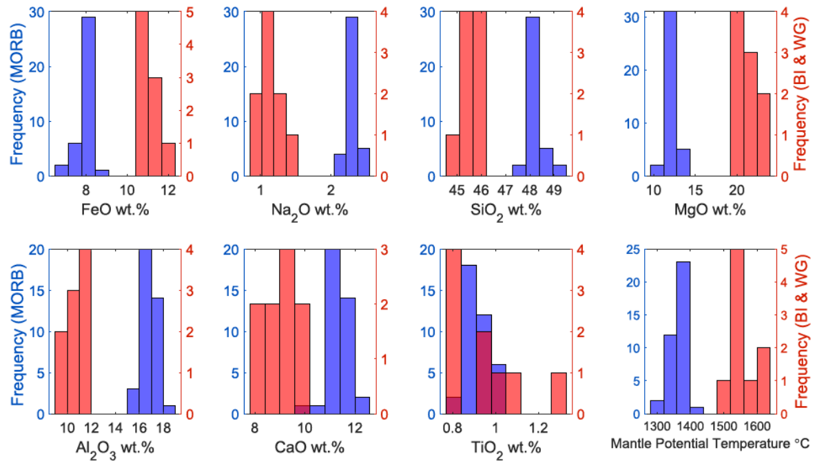
Figure 3. Histogram of calculated primary melt compositions for high-MgO (> 10 wt. %) MORB (blue) from the Siqueiros transform fault from Perfit et al. [1996] and Hays [2004] and primary melt compositions for Baffin Island (BI) and West Greenland (WG) lavas (red). The data in the histograms are consistent with hotter, deeper melting at BI-WG compared to MORB. BI-WG samples have been filtered for crustal assimilation so that all lavas plotted have Nb/Th > 13, Ce/Pb > 20, and MgO > 10 wt. %; high-Ba/Th (>100) samples from West Greenland are not considered as they are considered altered by mantle metasomatism. Primary melts are calculated using PRIMELT3 from Herzberg and Asimow [2015] using \text{Fe}_2\text{O}_3/\text{TiO}_2 = 0.5 and accumulated fractional melting. Mantle potential temperatures calculated with PRIMELT3 software are also shown. The number of samples for BI-WG (N=9) is greater here than in isotope plots because isotopes are not required for petrologic analyses.
