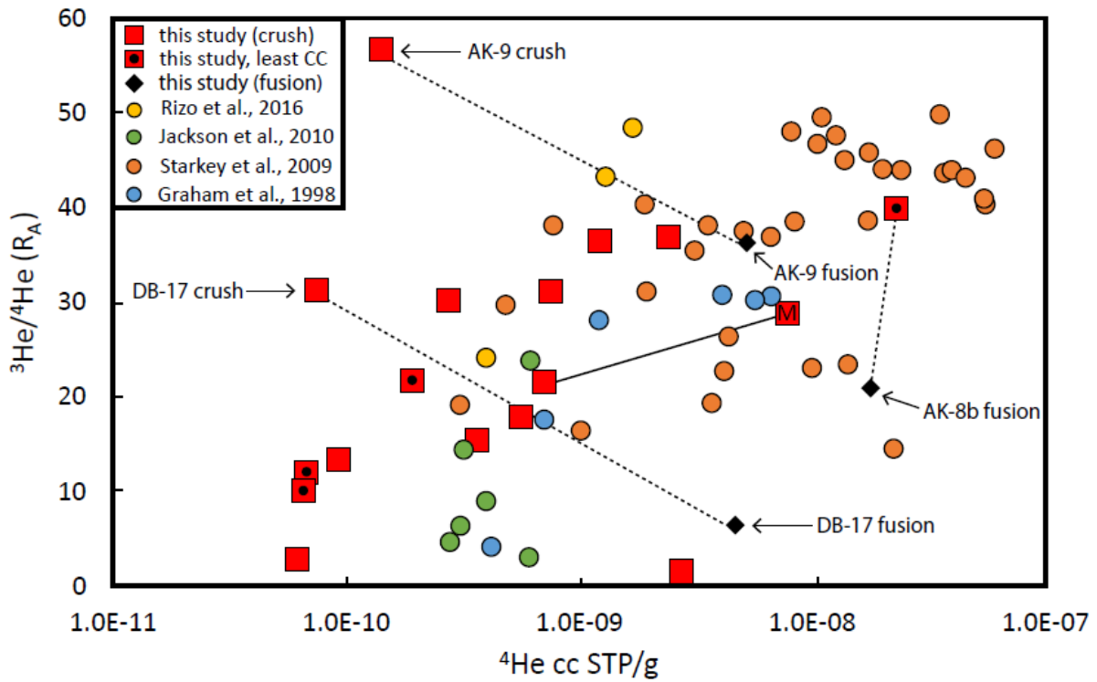
Figure 11. Helium isotopic compositions compared to ^4\text{He} concentrations for Baffin Island and West Greenland magmatic olivines. Samples with lower helium concentrations tend to have lower ^3\text{He}/^4\text{He} , possibly due to greater sensitivity to post-eruptive radiogenic ingrowth of ^4\text{He} . The dashed lines connect the olivine crush experiment data to the respective fusion results for three different samples. The solid line connects a crush experiment on a single olivine megacryst (denoted by an “M” in the symbol) to the crush experiment for multiple smaller olivine phenocrysts from the same lavas (AK-13). In the key, CC signifies crustal contamination.
