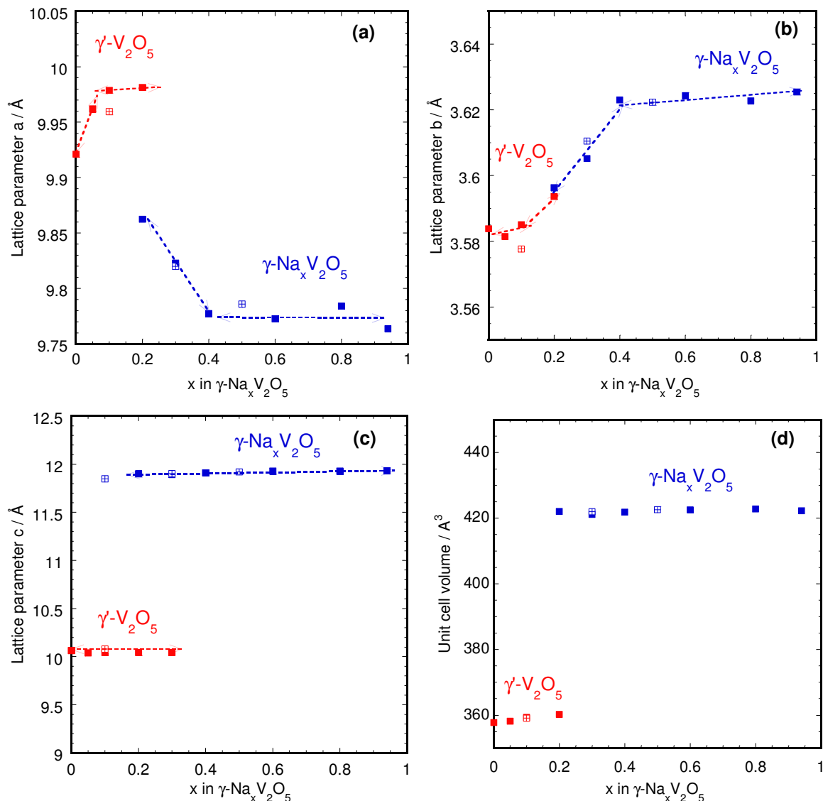
Figure 4. Evolution of (a-b-c) unit cell parameters and (d) volume of the phases formed during the first discharge-charge cycle of BM-30 \gamma' - V_2O_5 in 1M NaClO_4 PC + FEC (2% vol.): \blacksquare discharge \boxplus charge ( 0 \leq x \leq 0.94 ).
