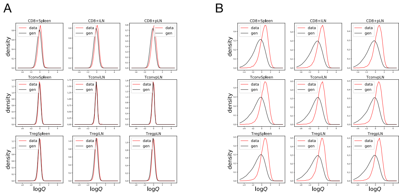
FIG. S5: (A) Distribution of \log Q of inferred models starting from an empirical baseline \mathcal{G} and (B) Distribution of \log Q of inferred models starting from P_{\text{gen}} as a baseline.
