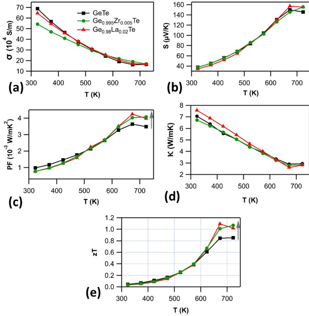
Figure 7. Temperature-dependent (a) electrical conductivity ( \sigma ), (b) Seebeck coefficient ( S ), (c) power factor ( PF = S^2\sigma ), (d) total thermal conductivity ( \kappa ), (e) figure of merit ( zT ) for \text{Ge}_{0.995}\text{Zr}_{0.005}\text{Te} and \text{Ge}_{0.98}\text{La}_{0.02}\text{Te} compounds.
