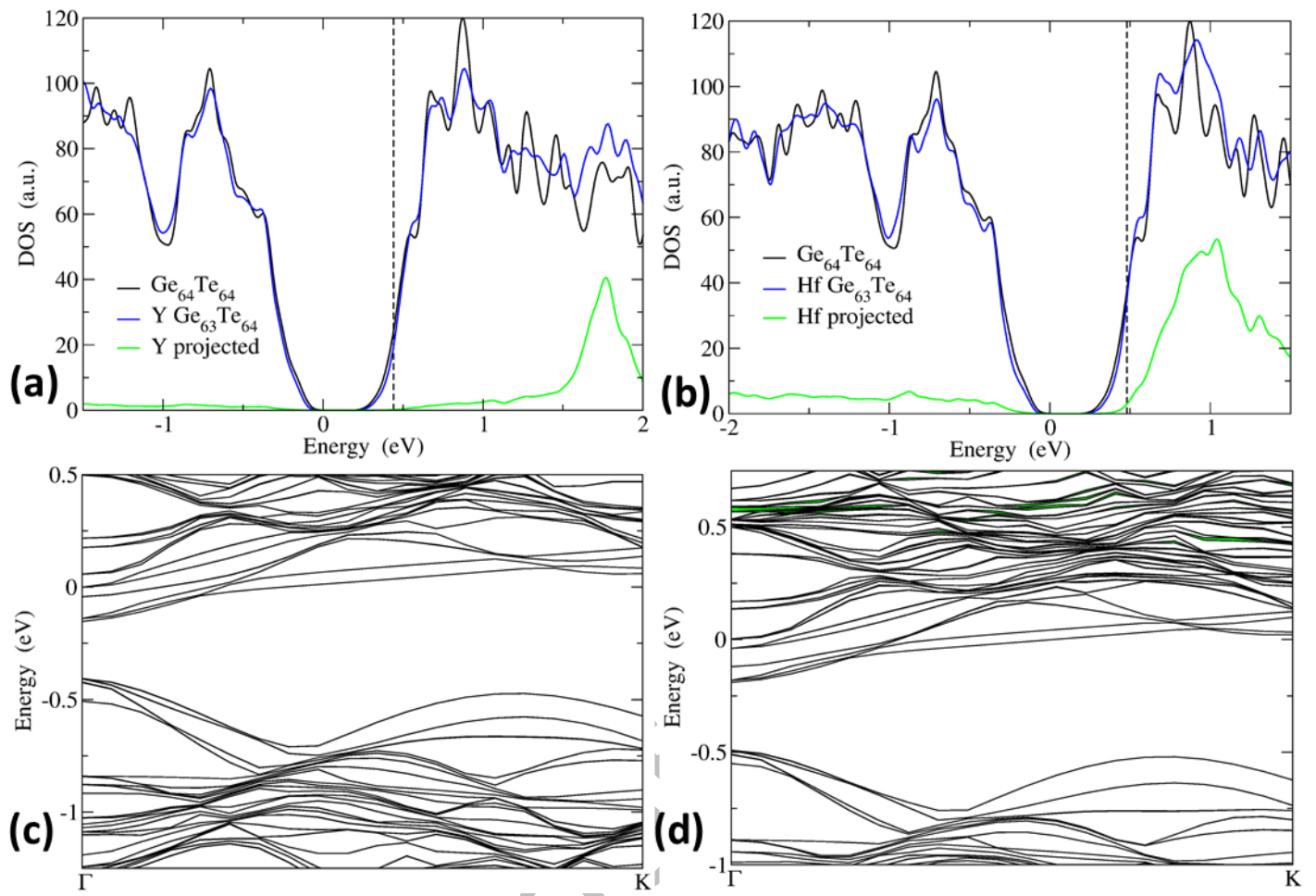
Figure 6. First-principles computed DOS for (a) \text{YGe}_{63}\text{Te}_{64} and (b) \text{HfGe}_{63}\text{Te}_{64} , and computed band structures for (c) \text{YGe}_{63}\text{Te}_{64} and (d) \text{HfGe}_{63}\text{Te}_{64} cubic models. Additional figure captions (regarding E_F , additional Gaussian smearing, and projection of the wave function) given in Figures 4 and 5, apply also here.
