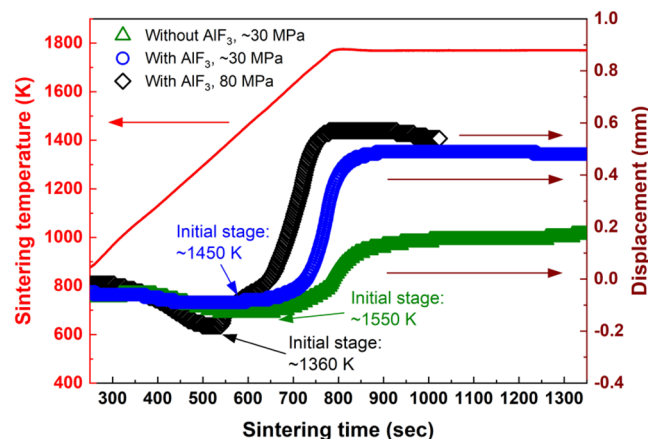
Figure 4. Densification behavior of Y_xAl_{1-y}B_{14} sintered without AlF_3 under \sim 30 MPa, with AlF_3 under \sim 30 MPa and with AlF_3 under 80 MPa. To investigate the effect of AlF_3 to densification, same amount of mixture and same graphite die and spacers were used.
