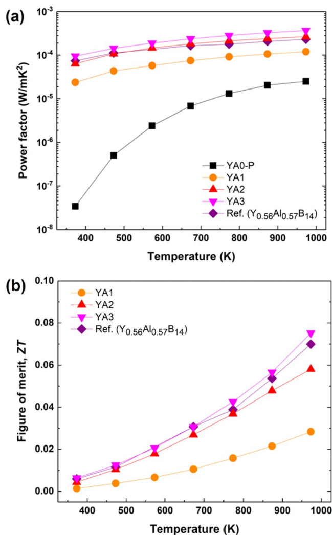
Figure 16. (a) Power factor and (b) figure of merits for \text{Y}_x\text{Al}_{1-x}\text{B}_{14} ( x \sim 0.64 ) samples prepared by reactive SPS, which are compared with the reported value of \text{Y}_{0.56}\text{Al}_{0.57}\text{B}_{14} 44 .
