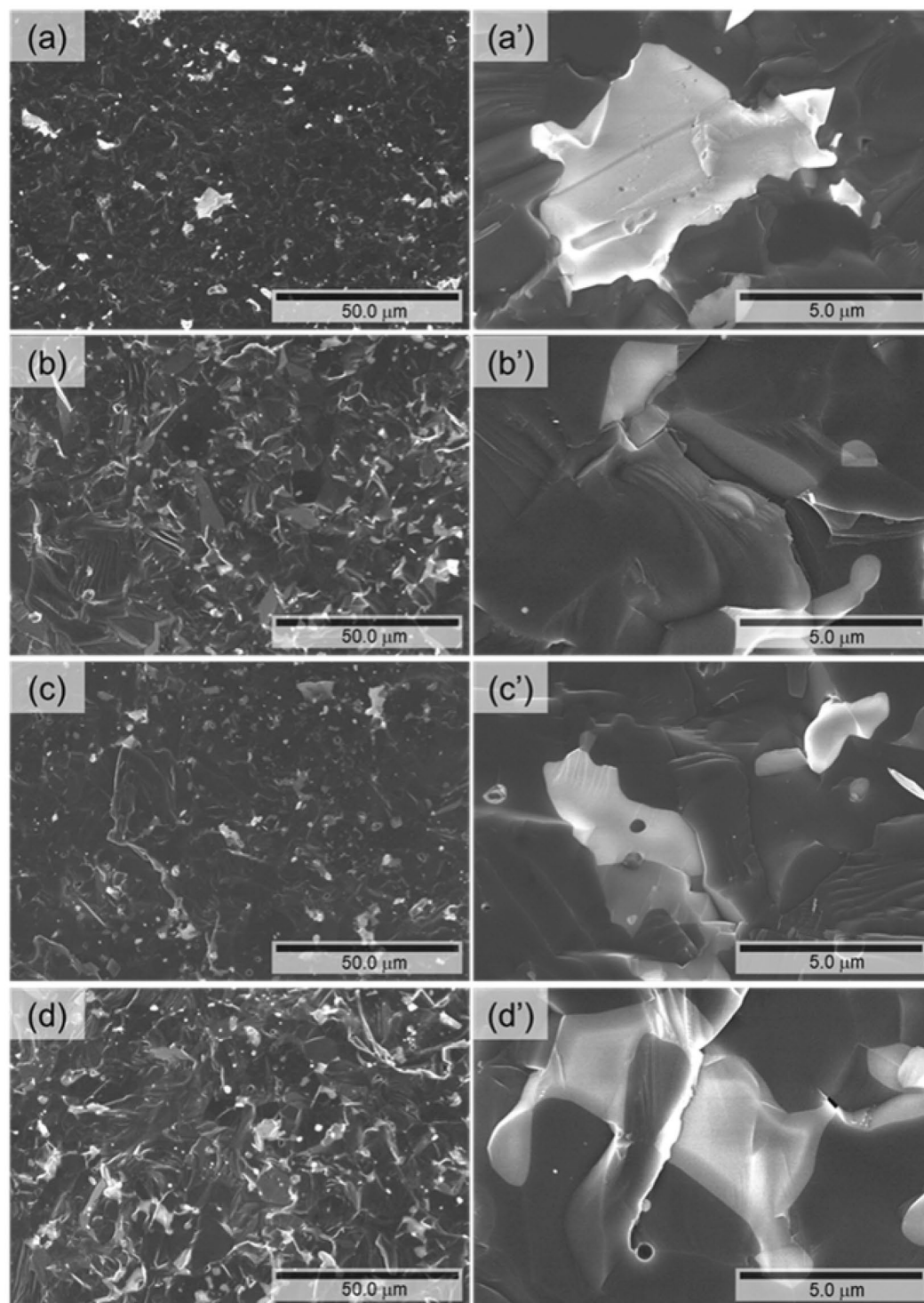
Figure 13. SEM images of fracture surface for Y_xAl_{14}B_{14} samples prepared by reactive SPS, (a,a') YA0-P, (b,b') YA1, (c,c') YA2 and (d,d') YA3.
