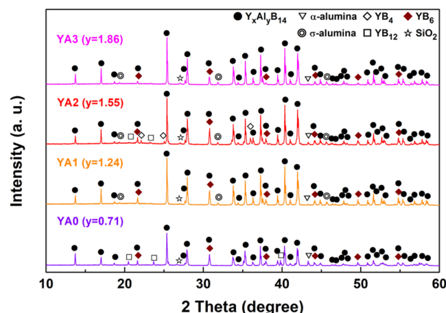
Figure 5. XRD patterns of YA0, YA1, YA2 and YA3 composition ( Y_{0.62}Al_yB_{14} ; y = 0.71\text{--}1.86 ) samples prepared by reactive SPS with AlF_3 addition. The samples were sintered at 1773 K under uniaxial pressure of \sim 30 MPa in a reduced Ar atmosphere for 1 h.
