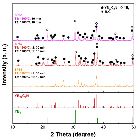
Fig. 2. The XRD patterns of the SPS1, SPS2 and SPS3 samples prepared with different nitrogen treatment temperature ( T_1 ) by reactive SPS.
