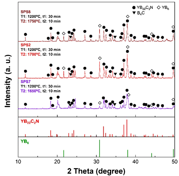
Fig. 4. The XRD patterns of the SPS7, SPS2 and SPS8 samples prepared with different sintering temperature (T2) by reactive SPS.
