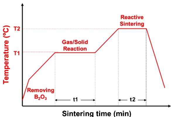
Fig. 1. The sintering schedule for synthesis of \text{YB}_{22}\text{C}_2\text{N} by reactive SPS.
