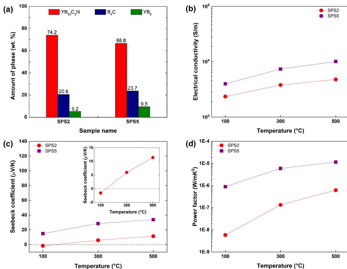
Fig. 6. (a) The amount of \text{YB}_{22}\text{C}_2\text{N} , \text{B}_4\text{C} and \text{YB}_6 phases, (b) the electrical conductivities, (c) Seebeck coefficients and (d) the power factors of the SPS2 and SPS5 samples.
