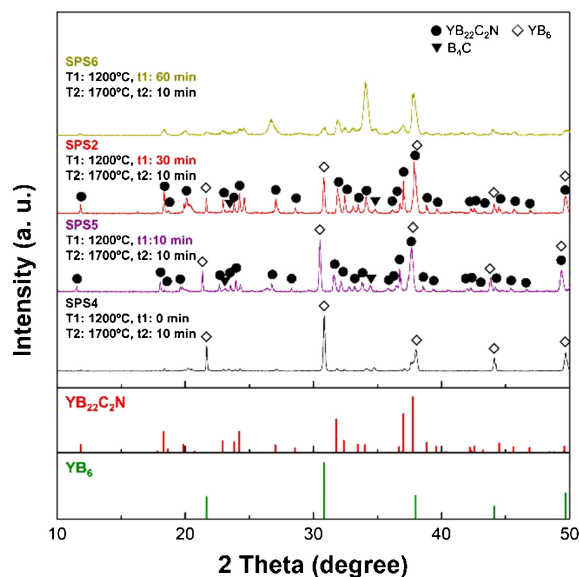
Fig. 3. The XRD patterns of the SPS4, SPS5, SPS2 and SPS6 samples prepared with different nitrogen treatment time ( t_1 ) by reactive SPS.
