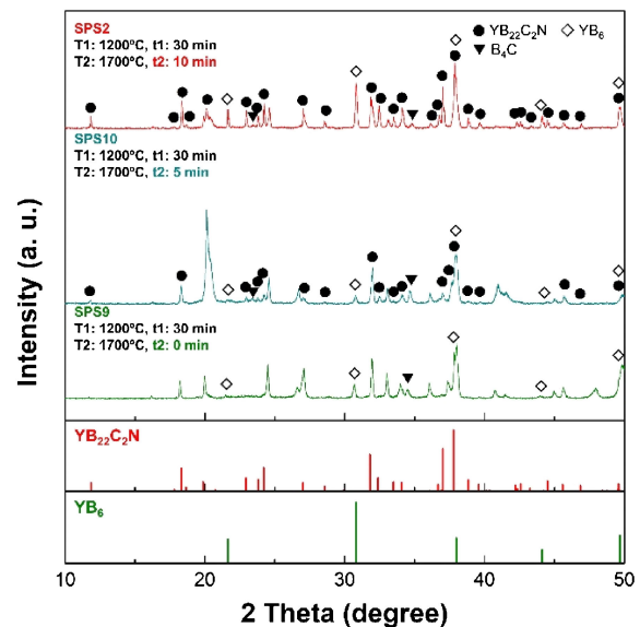
Fig. 5. The XRD patterns of the SPS9, SPS10 and SPS2 samples prepared with different sintering time ( t_2 ) by reactive SPS.
