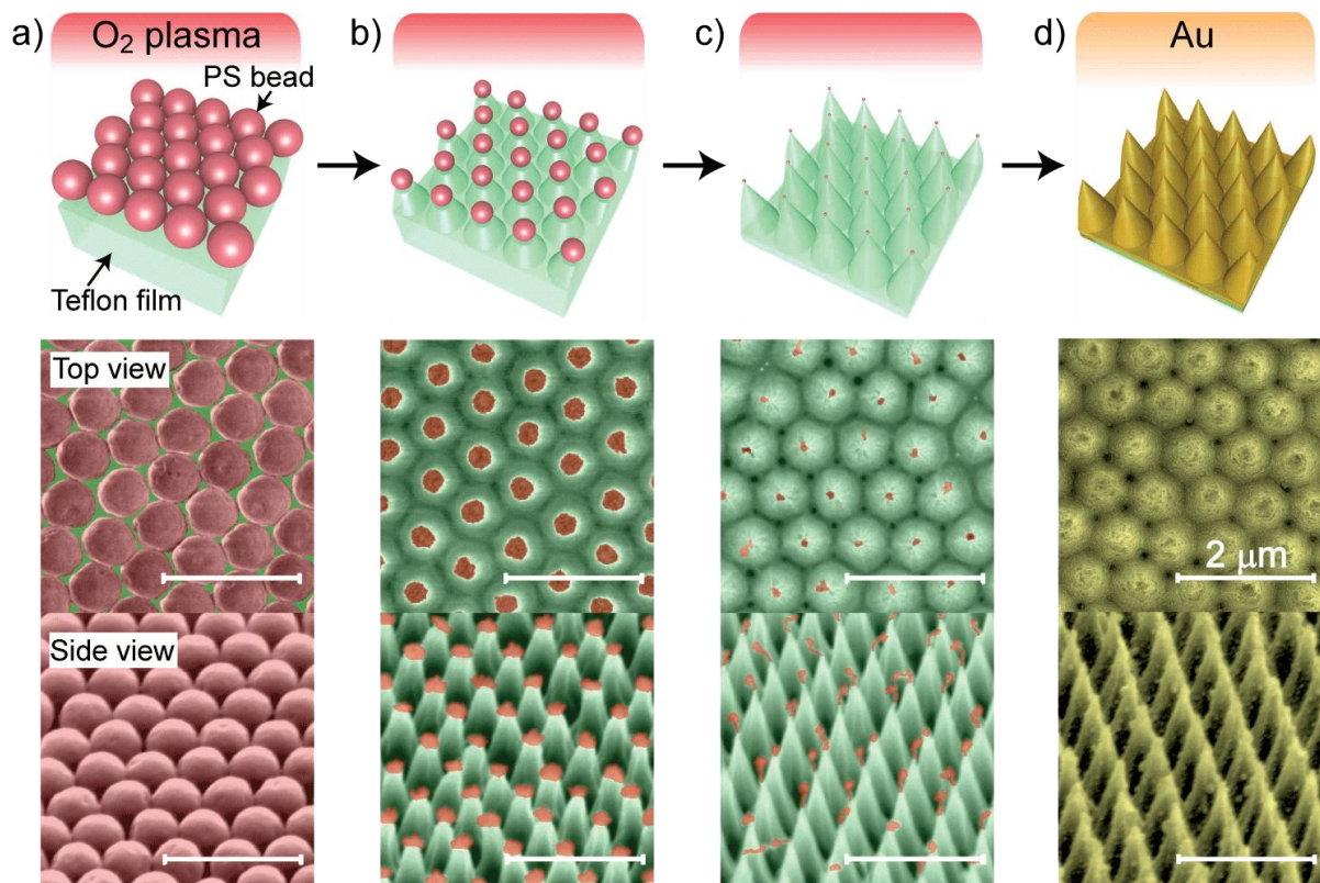
Figure 1. a-d) Schematic illustration of the fabrication process (top row) and colored SEM images of the corresponding samples in both top (middle row) and tilted (bottom row) views. a) Fabrication of a PS bead monolayer on a flexible teflon film. b-c) Formation of nanocone arrays by simultaneous plasma etching of PS beads and teflon film. d) Deposition of gold thin film on the teflon nanocone array. In all the SEM images, the scalebars indicate 2 \mu\text{m} .
