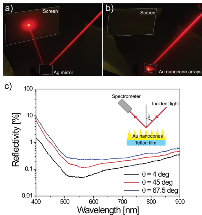
Figure 6. Photographs showing the laser beam path reflected by a) a silver mirror and b) a gold nanocone array. c) Reflectivity spectra from gold nanocone arrays at different angles of incidence, 4^\circ (black), 45^\circ (red) and 67.5^\circ (blue). The inserted schematic shows the optical setup used for reflectivity measurement.
