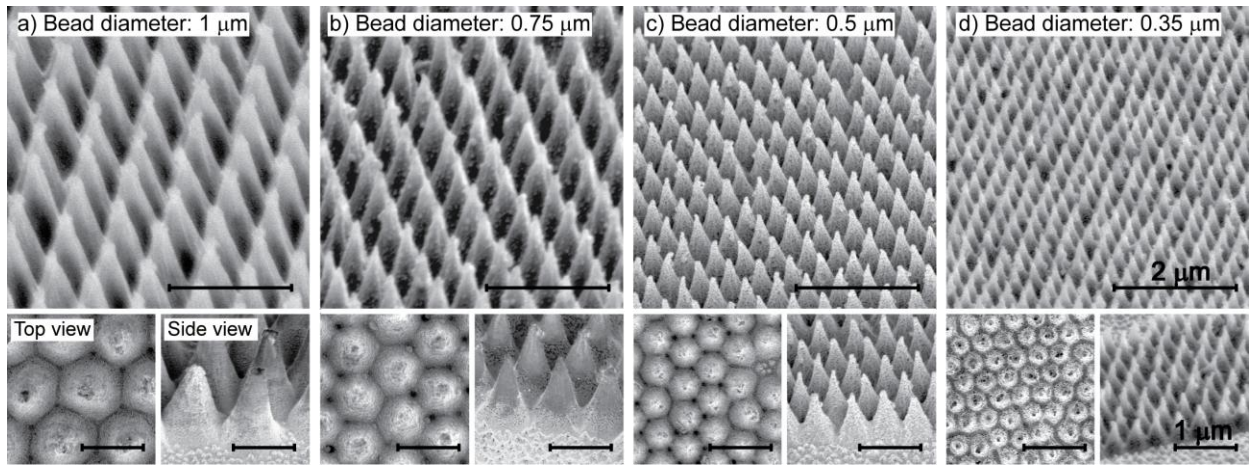
Figure 3. SEM images of nanocone arrays fabricated with PS beads with different diameter, a) 1 μm, b) 0.75 μm, c) 0.5 μm and d) 0.35 μm. The top row shows large tilted views. In the bottom row, left and right images show top view and side view of nanocones, respectively. In all the top and bottom SEM images, the scalebars indicate 2 μm and 1 μm, respectively.
