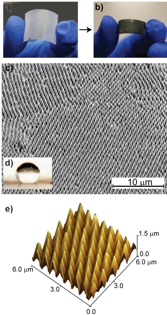
Figure 2. Photographs of the nanocone arrays on teflon film a) before and b) after coating with 50 nm thick gold layer. c) SEM image of the gold nanocone array in tilted view. d) Photograph of a water droplet on gold nanocone array showing the hydrophobicity of the surface. e) Three-dimensional AFM image of the gold nanocone array.
