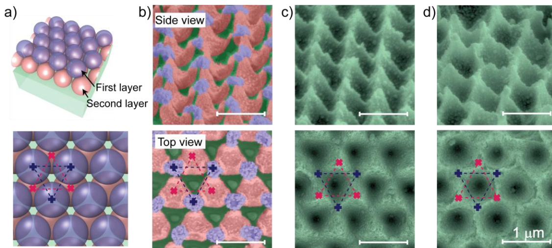
Figure 4 a) Schematic representation of a colloidal bilayer structure (top: tilted view, bottom: top view). b-d) Colored SEM images of colloidal bilayer structures after 3, 6 and 12 min O 2 plasma treatment, respectively. The areas corresponding to the first and second PS beads layers and teflon film are colored following the schematic drawing. In all the SEM pictures, crosses indicate the central position of PS beads at first (blue) and second (magenta) layers and the scalebars indicate 1 μm.
