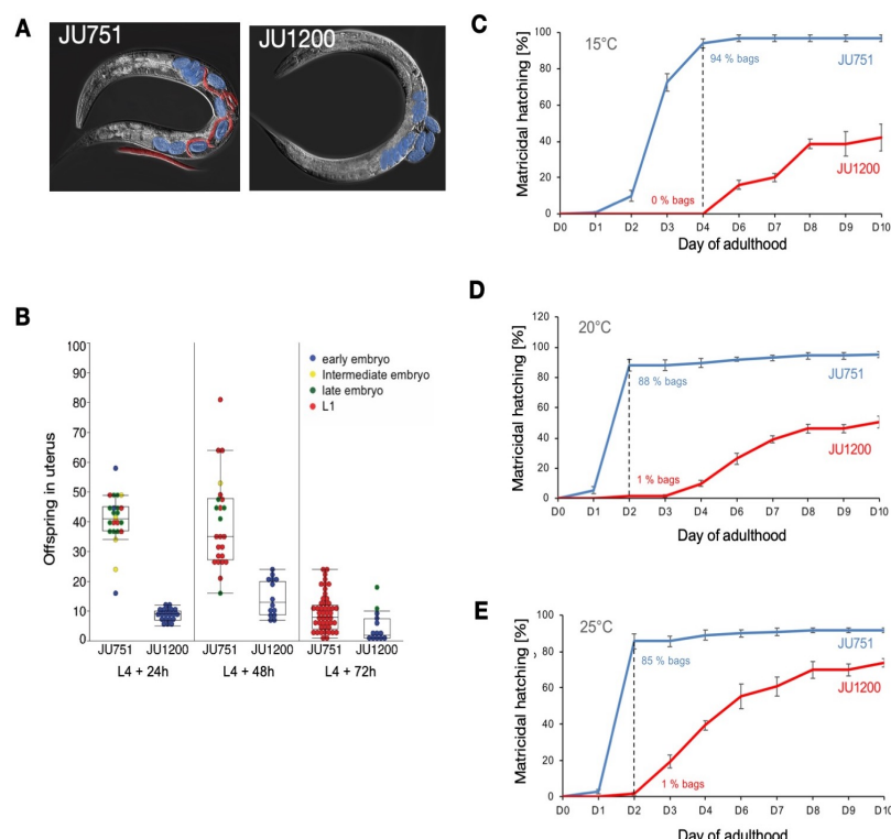
Fig. S1. Constitutive matricidal hatching in JU751
