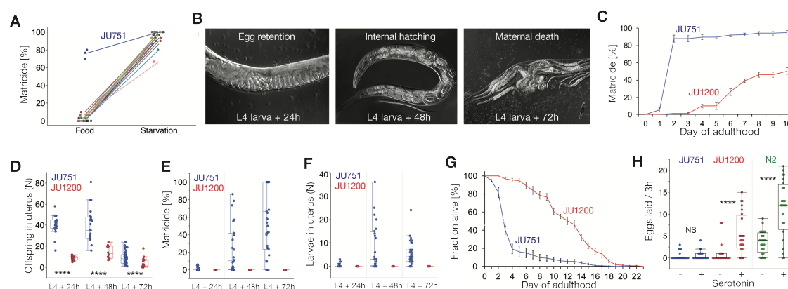
Fig. 1. Natural variation in plasticity of C. elegans matricidal hatching
