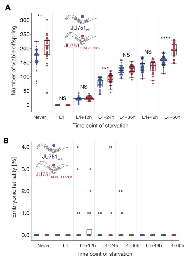
Fig. S12. Fitness consequences KCNL-1 V530L in variable environments
