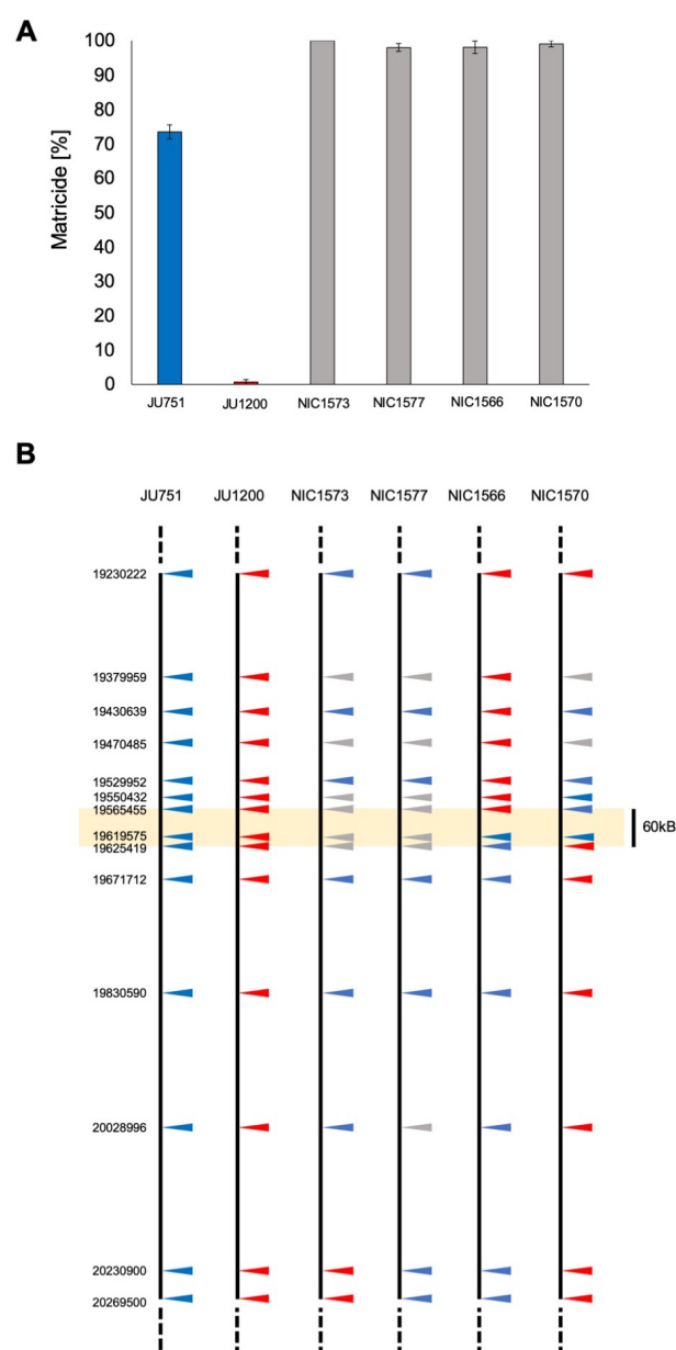
Fig. S7. Phenotyping of near-isogenic lines and fine-mapping of QTL region
