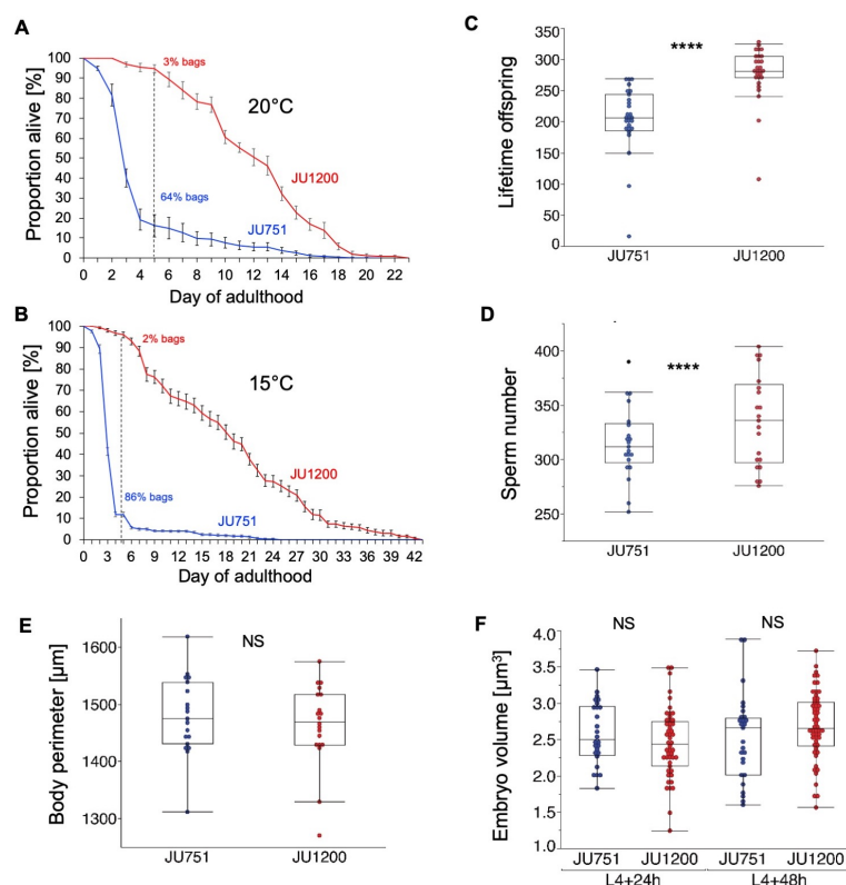
Figure S3. Life history differences between JU751 and JU1200
