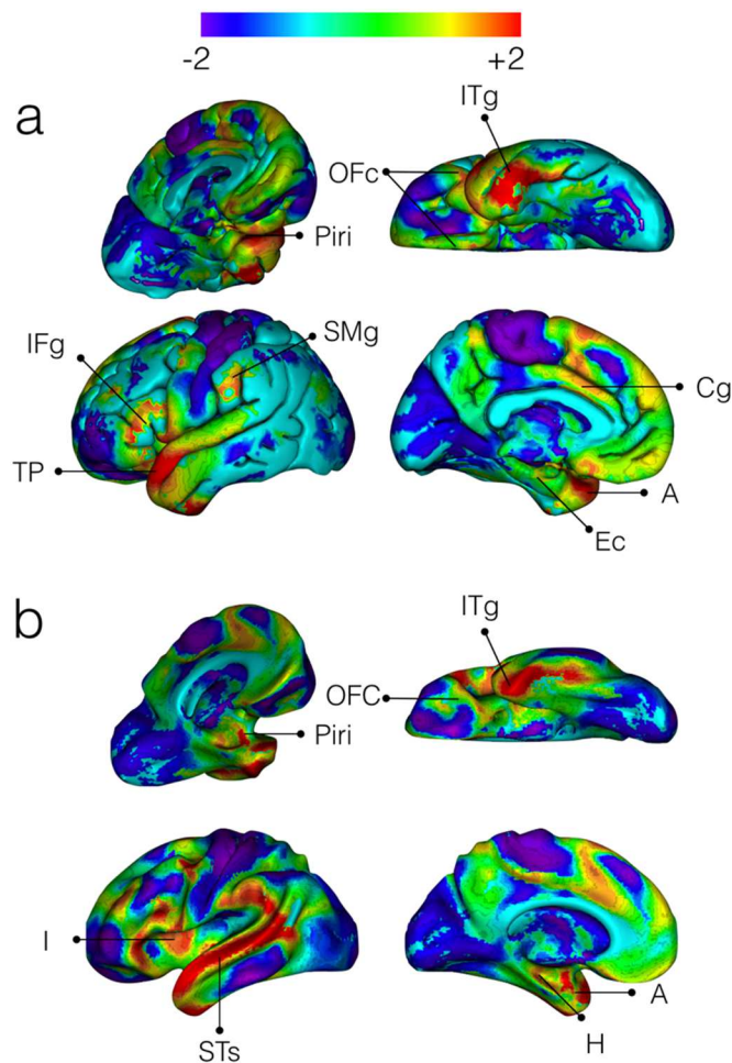
Figure 2: The fifth gradient of functional connectivity in the human brain. a) Shows the cortical surface representation of the gradient while b) demonstrates the inflated white matter surface. ITg: Inferior Temporal gyrus; OFc: Orbitofrontal cortex; Piri: Piriform cortex; IFg: Inferior Frontal gyrus; TP: temporal pole; SMg: Supramarginal gyrus; Cg: Cingulate gyrus; I: Insula; STs: Superior Temporal sulcus; Ec: Entorhinal cortex; A: Amygdala; H: Hippocampus
