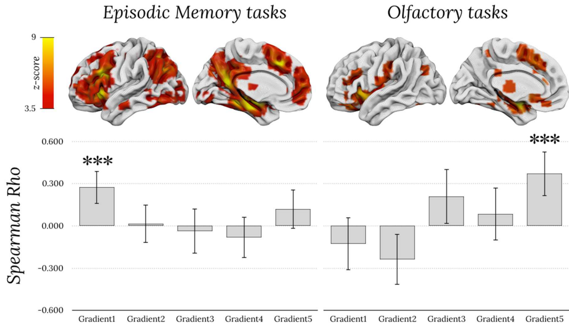
Figure 1: Spearman rank correlations between fMRI meta-analytic maps of episodic memory tasks (left), olfactory tasks (right), and values of the five gradients. Top row corresponds to meta-analytic activations maps from neurosynth. Error bars corresponds to 95% confidence intervals. *** indicates p < 0.001 and is significant after Bonferroni correction for multiple comparisons.
