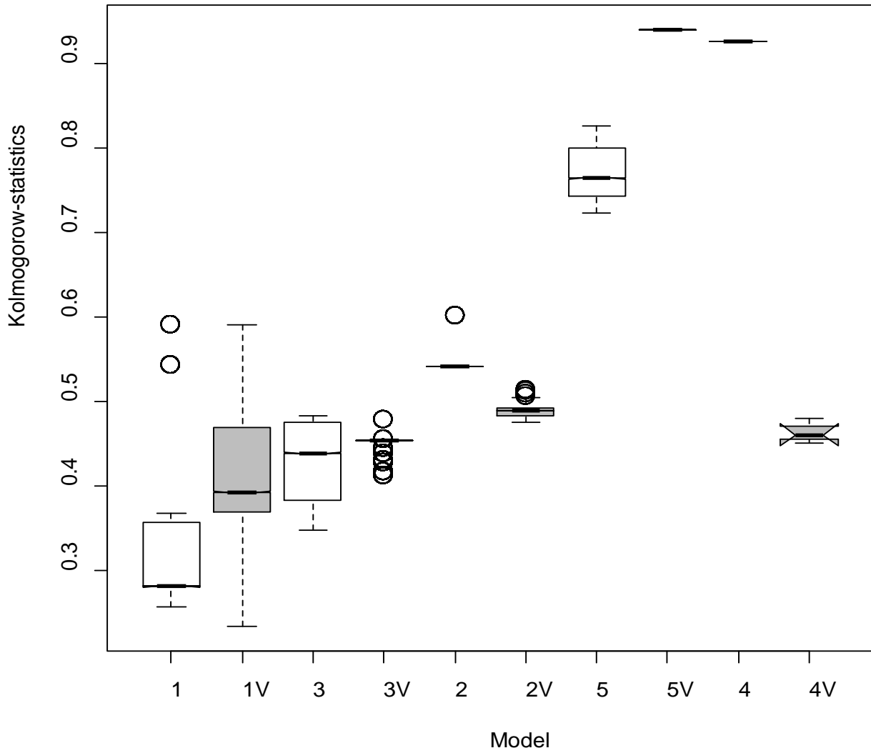
525 Figure 3. The test values of the Kolmogorow-Smirnow statistics when comparing the predicted cover 526 distribution for each model with the observed empirical cover distribution. The full model is identified by 527 its number and the variable selected model by the suffix "V" (gray color). Model numbers refer to Table 528 2.
