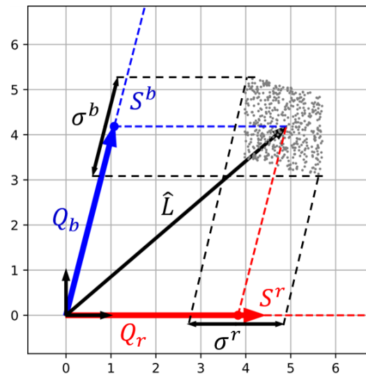
Figure 13. Projection of the uncertainty volume onto contravariant coordinates. Uncertainty in spectral reconstruction is given by contravariant noise \sigma^r and \sigma^b . When the angle between channel is smaller, the contravariant coordinates and SNR decrease. Spectral reconstruction becomes “more noisy”.
