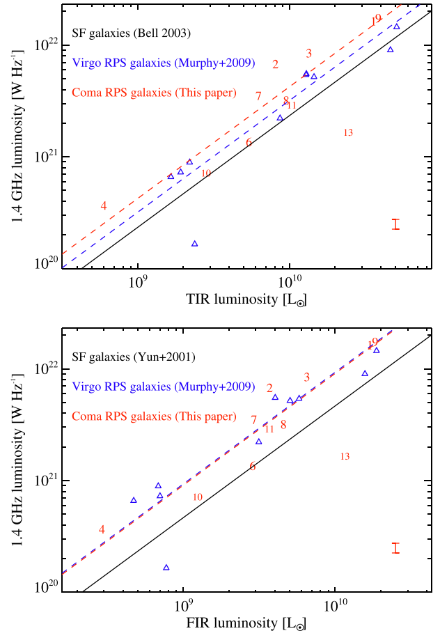
Figure 7. The 1.4 GHz luminosity versus TIR (top plot) and FIR (bottom plot) luminosity for the RPS galaxies. The galaxies in the Coma cluster are in red and those in the Virgo cluster (Murphy et al. 2009) are in blue. Each number indicates a galaxy as listed in Table 2. The mean ratios of 1.4 GHz to TIR (FIR) for RPS galaxies in the Coma cluster and in the Virgo cluster are shown as red and blue dashed lines, respectively. The relations between the 1.4 GHz continuum and TIR (Bell 2003) or FIR (Yun, Reddy & Condon 2001) for star-forming galaxies are also shown as black solid lines.
