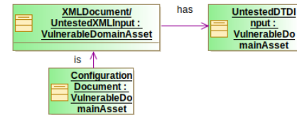
Fig. 8: An Excerpt of Vulnerable Domain Assets
