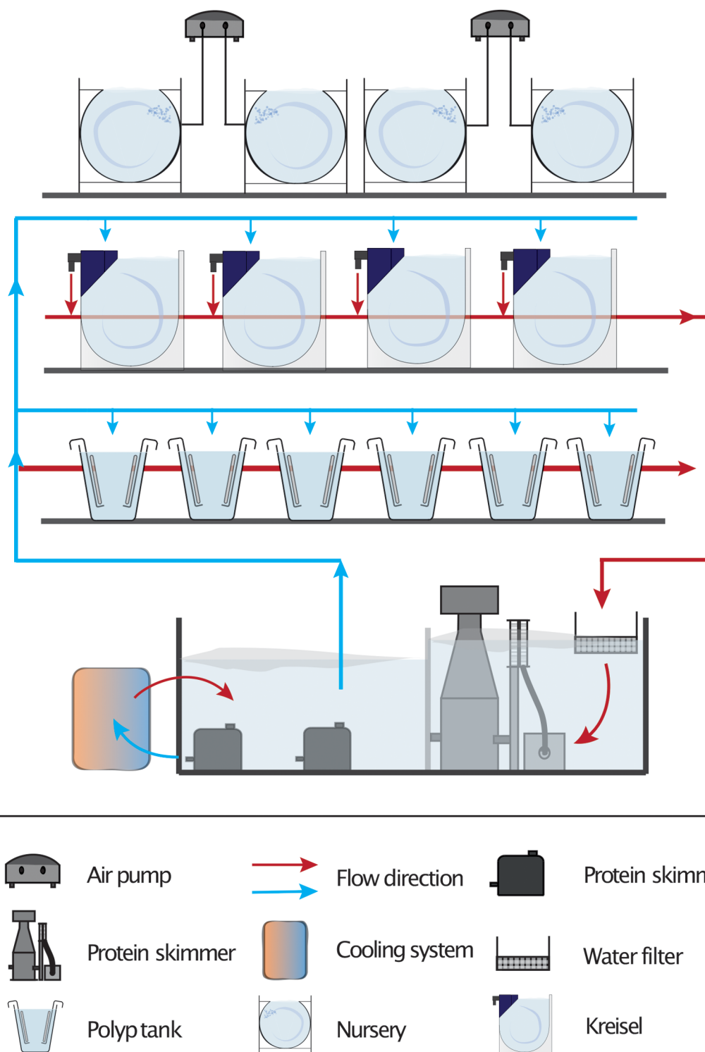
Fig. 3. Culture system in the laboratory. Both Kreisel tanks (large medusae) and polyp tanks are integrated in a closed-circuit water aquaculture system. Water is supplied to each tank from the reservoir (50–80 liters) by a submerged pump. Excess artemia, food leftovers or released Clytia jellyfish are primarily removed by a nylon mesh (200 \mu\text{m} ) or filter pad (50 \mu\text{m} ), then by protein skimmer, before the water returns to the reservoir. The temperature is adjusted by water chiller/heater. The salinity is measured every 2–3 days and adjusted by adding deionized water. Roughly half of the water in the reservoir tank is replaced every 2 months.
