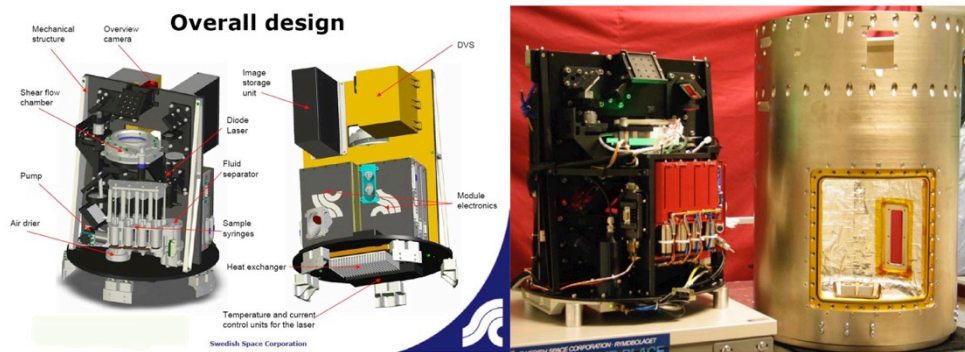
Figure 7: The BIOMICS module developed by SSC with a contribution of Lambda-X for the holographic microscope. Left: overall design. Right: picture of the module and its payload housing with the hatch open.
