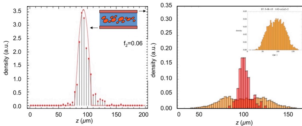
Figure 9: Some results from MASER 11 and MASER 12 [13,18]. Left: the steady distribution of a monodisperse vesicle sample allows the determination of shear-induced diffusion coefficients (inset: sketch of the experiment). Right: steady distribution for a bi-disperse suspension of vesicles in MASER 12 (yellow: small vesicles with average radius 10 μm, red: big vesicles with average radius 20 μm). The double peak for small vesicles (to be compared to the unique, smooth peak when they are alone as show in the insert) reveals segregation phenomena in the flow of polydisperse cellular suspensions.
