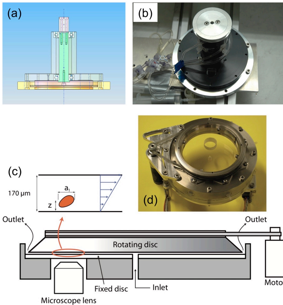
Figure 2: Two versions of the shear flow chamber developed for microgravity experiments. (a) and (b): sketch and picture of the prototype designed at LIPhy and tested in the parabolic flights campaigns of spring 2006 (ESA) and September 2006 (CNES); (c) and (d): sketch and picture of the shear flow chamber designed and developed by SSC and used in the MASER 11 (2008) and MASER 12 (2012) sounding rocket flights and in ESA and CNES parabolic flight campaigns since 2007 for various experiments on vesicles and red blood cell dynamics (from [12]).
