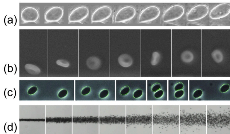
Figure 1: Basic phenomena of vesicle and red blood cell dynamics in confined flows. (a) Unbinding and lift of a vesicle in shear flow; (b) migration of a red blood cell (from [7]); (c) repulsive hydrodynamic interaction in a pair of vesicles in shear flow (from [8]); (d) shear-induced diffusion of red blood cells in a channel (from [9]).
