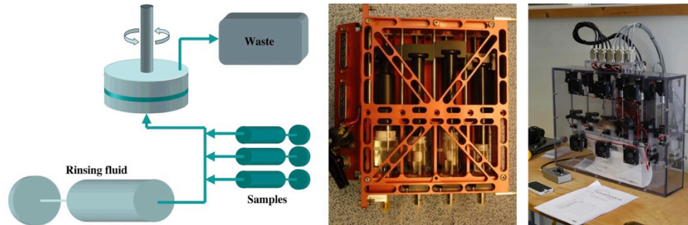
Figure 4: Multi-channel injection system. Left: sketch of the system; Middle: Multi-channel syringe pump with embedded stirring system designed by SSC for the BIOMICS module in MASER rockets; Right: Similar system developed at LIPhy for recent parabolic flight campaigns (2017-2019).
