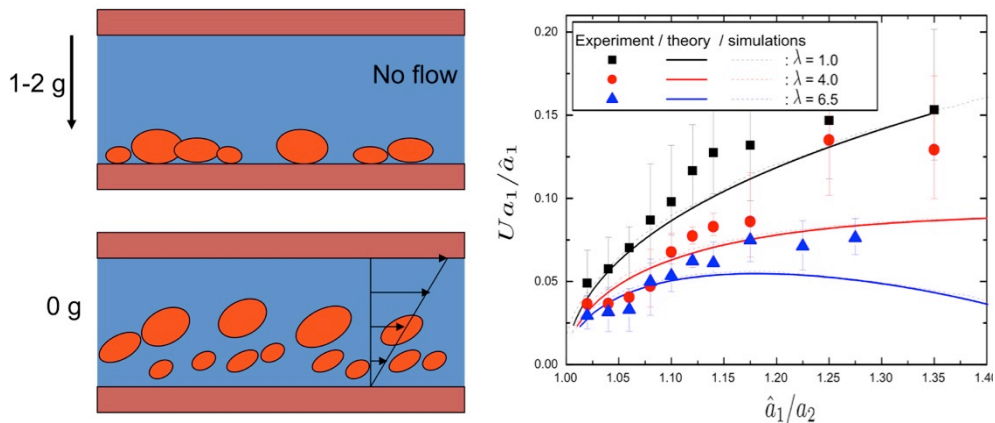
Figure 5: Experiments on the lift of vesicles in shear flow near a wall performed in parabolic flights for the determination of lift coefficients. The motor of the shear flow chamber is stopped during normal and hyper gravity phases (1-2 g) to allow sedimentation of vesicles on the bottom wall and the fluid is sheared during microgravity phases only to study the resuspension of vesicles. Results show a strong dependency of the dimensionless lift velocity U on vesicle parameters such as viscosity ratio \lambda and elongation a_1/a_2 (from [13])
