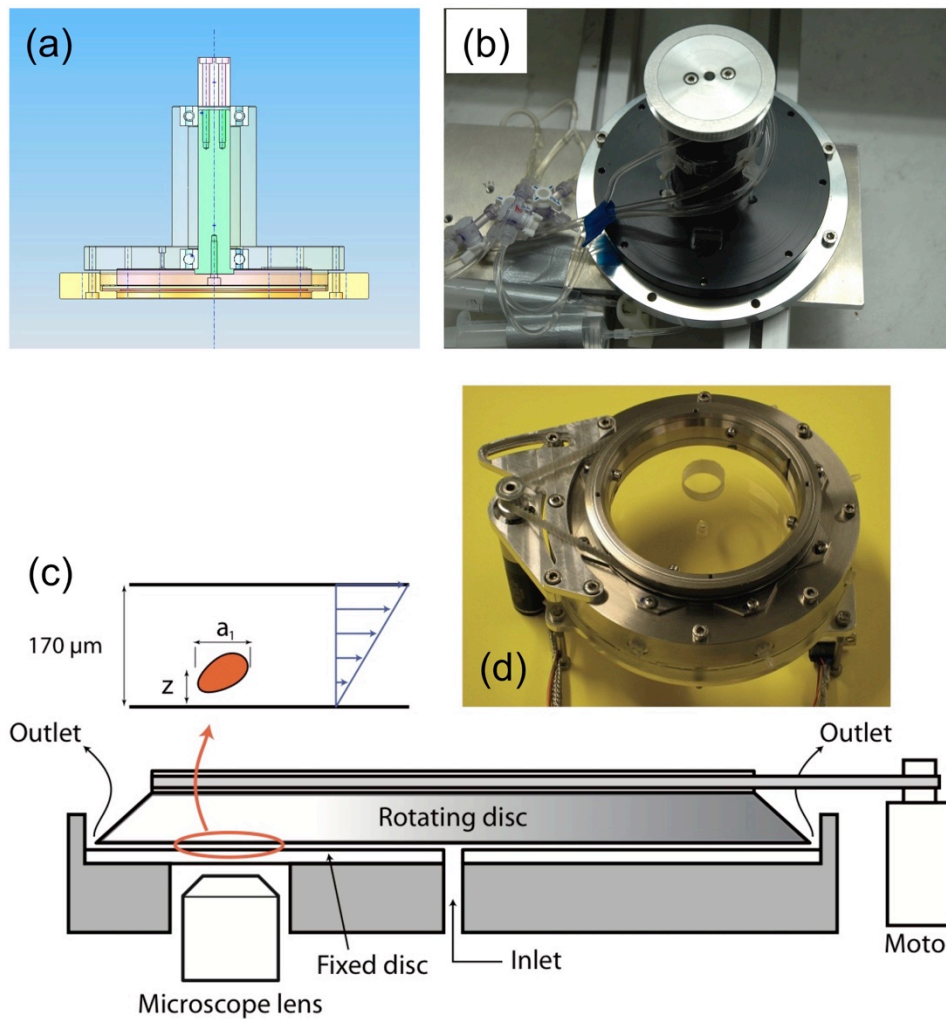
Figure 2: Two versions of the shear flow chamber developed for microgravity experiments. (a) and (b): sketch and picture of the prototype designed at LIPhy and tested in the parabolic flights campaigns of spring 2006 (ESA) and September 2006 (CNES); (c) and (d): sketch and picture of the shear flow chamber designed and developed by SSC and used in the MASER 11 (2008) and MASER 12 (2012) sounding rocket flights and in ESA and CNES parabolic flight campaigns since 2007 for various experiments on vesicles and red blood cell dynamics (from [12]).
