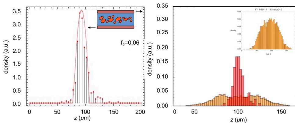
Figure 9: Some results from MASER 11 and MASER 12 [13,18]. Left: the steady distribution of a monodisperse vesicle sample allows the determination of shear-induced diffusion coefficients (inset: sketch of the experiment). Right: steady distribution for a bi-disperse suspension of vesicles in MASER 12 (yellow: small vesicles with average radius 10 \mu\text{m} , red: big vesicles with average radius 20 \mu\text{m} ). The double peak for small vesicles (to be compared to the unique, smooth peak when they are alone as show in the insert) reveals segregation phenomena in the flow of polydisperse cellular suspensions.
