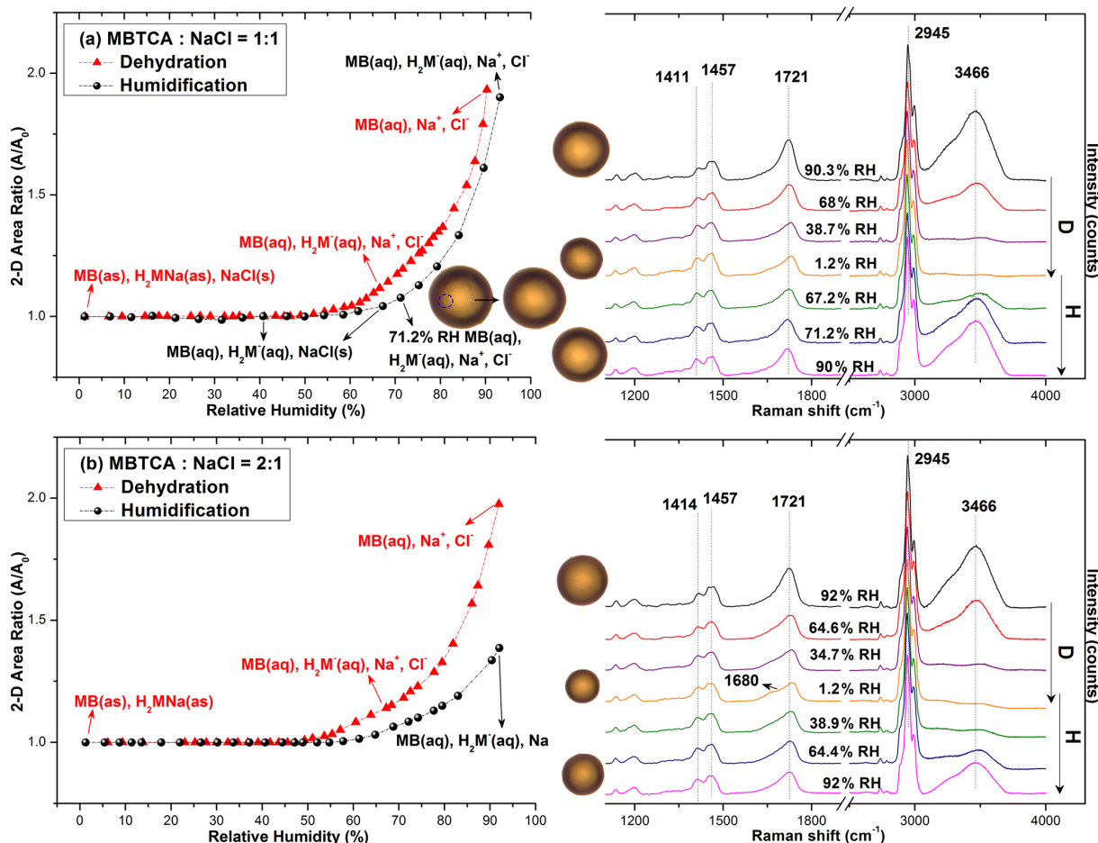
Figure 4. Hygroscopic curves, corresponding optical images, and Raman spectra at specific RHs of MBTCA:NaCl = (a) 1:1 and (b) 2:1. The recorded transition RHs during the dehydration (D) and humidification (H) processes and the chemical compositions of the mixtures at certain RHs are marked with arrows in the hygroscopic curves. The phase notations shown in parentheses are s – solid, aq – aqueous, and as – amorphous solid.
