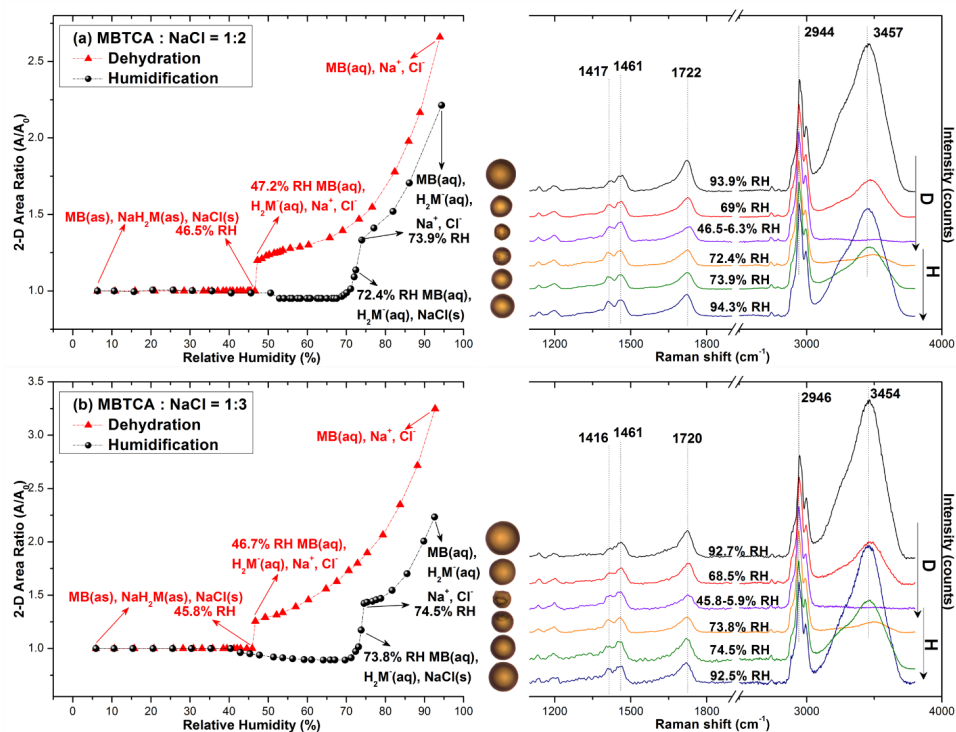
963 Figure 5. Hygroscopic curves, corresponding optical images, and Raman spectra at specific RHs of MBTCA:NaCl = (a) 1:2 and (b) 1:3. 964 The recorded transition RHs during the dehydration (D) and humidification (H) processes and the chemical compositions of the mixtures 965 at certain RHs are marked with arrows in the hygroscopic curves. The phase notations shown in parenthesis are s=solid; aq=aqueous; 966 and as=amorphous solid.
