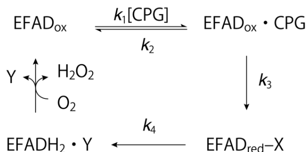
Scheme 1. Catalytic cycle of MSOX for CPG. 15
