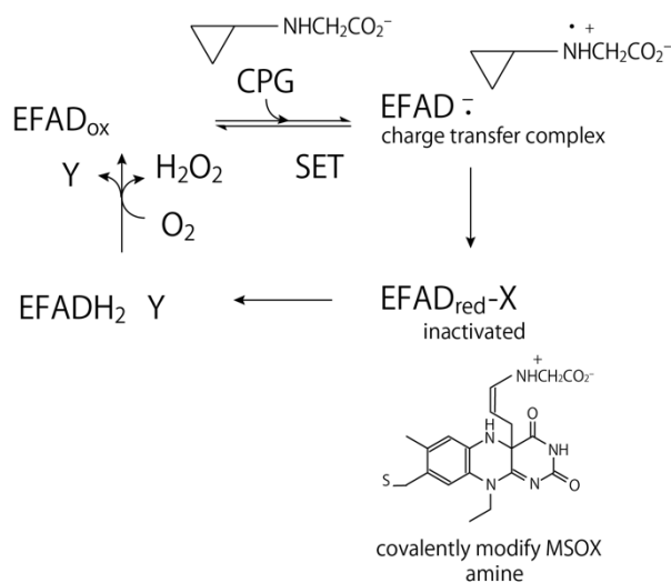
Scheme 2. Proposed CPG states in MSOX. 16
