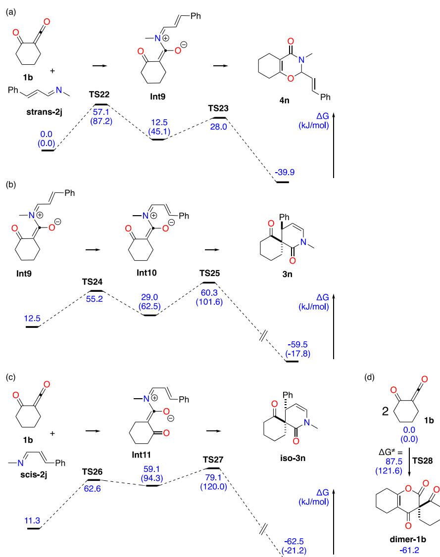
Figure 5. Free Gibbs energy profiles computed at 298 K (DFT, B3LYP-D3/6-311++G(d,p)) of the aza-Diels–Alder reactions between the α-oxoketene 1b and the 1-azadiene 2j . Free Gibbs energies noted between parentheses were computed at 473 K.
