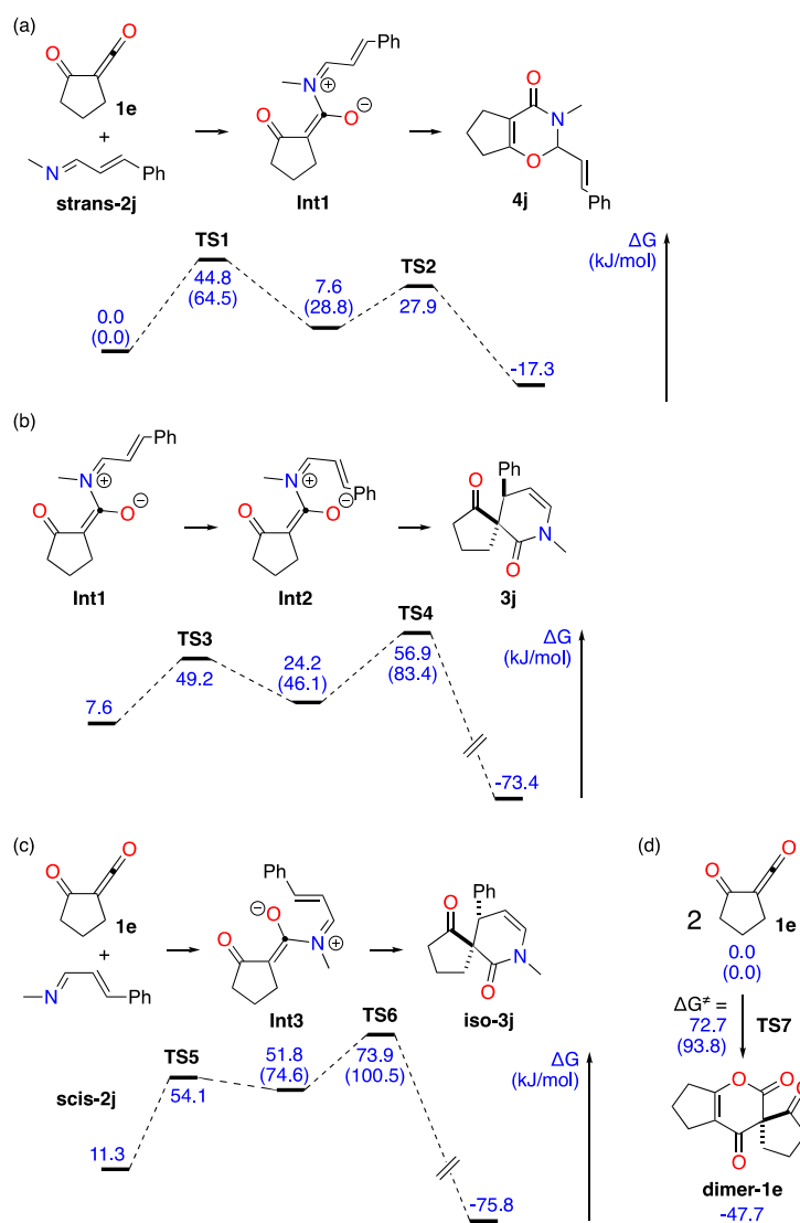
Figure 1. Free Gibbs energy profiles computed at 298 K (DFT, B3LYP-D3/6-311++G(d,p)) of the aza-Diels–Alder reactions between the \alpha -oxoketene 1e and the 1-azadiene 2j , and cyclodimerization of \alpha -oxoketene 1e . Free Gibbs energies noted between parentheses were computed at 413 K.
