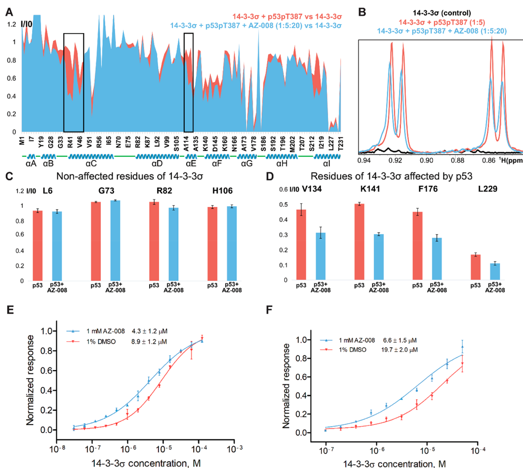
Figure 5. AZ-008 stabilizes the 14-3-3 \sigma /p53pT387 complex. (A) Plot of the intensity ratios I/I_0 (y-axis) of corresponding ^1\text{H} – ^{15}\text{N} correlation peaks in the 2D 14-3-3 \sigma ΔC17 spectra of, in red: the peptide-bound 14-3-3 \sigma ΔC17 (100 \mu\text{M} 14-3-3 \sigma in the presence of 500 \mu\text{M} p53pT387, I ) and free 14-3-3 \sigma (100 \mu\text{M} 14-3-3 \sigma I_0 ); in blue: corresponding to the peptide and fragment-bound 14-3-3 \sigma (100 \mu\text{M} 14-3-3 \sigma with 500 \mu\text{M} p53pT387 and 2000 \mu\text{M} AZ-008, I ) and free 14-3-3 \sigma (100 \mu\text{M} 14-3-3 \sigma , I_0 ) protein. Note that the boxed regions correspond to the same areas affected in Figure 4 D and therefore show that the binding site of the fragment is the same when the peptide is present or not. (B) ^1\text{H} NMR signals of the spectrum of 100 \mu\text{M} 14-3-3 \sigma (in black), 100 \mu\text{M} 14-3-3 \sigma in the presence of 500 \mu\text{M} p53pT387 (in red), and 100 \mu\text{M} 14-3-3 \sigma in the simultaneous presence of 500 \mu\text{M} p53pT387 and 2000 \mu\text{M} AZ-008 (in blue). The NMR signals correspond to the \text{H}\delta protons of L383 of the p53pT387 peptide. CSP in the peptide signals can be observed when AZ-008 is added to the solution containing the 14-3-3 \sigma /p53pT387 complex. (C,D) Plot of the ratios of the bound ( I )/free ( I_0 ) ^1\text{H} – ^{15}\text{N} TROSY-HSQC correlation peak intensities of individual resonances corresponding to residues of 100 \mu\text{M} 14-3-3 \sigma , remote from the interaction site (C) or close to the p53pT387 interaction site of (D), in the presence of 500 \mu\text{M} p53pT387 (in red) and 100 \mu\text{M} 14-3-3 \sigma in the simultaneous presence of 500 \mu\text{M} p53pT387 and 2000 \mu\text{M} AZ-008 (in blue). Error bars of I/I_0 ratios were calculated based on the maximum noise estimate of each spectrum. Note that the resonances corresponding to regions affected by the p53pT387 peptide binding were considerably more affected in the presence of AZ-008. (E) Titration of 14-3-3 \sigma to a fluorescently labeled p53pT387 peptide in the absence and presence of 1 mM of AZ-008. Shown are average and standard deviation of three independent experiments. (F) SPR measurement of 14-3-3 \sigma binding to immobilized p53pT387 peptide in the absence and presence of 1 mM AZ-008. Shown are average and standard deviation of three independent experiments.
