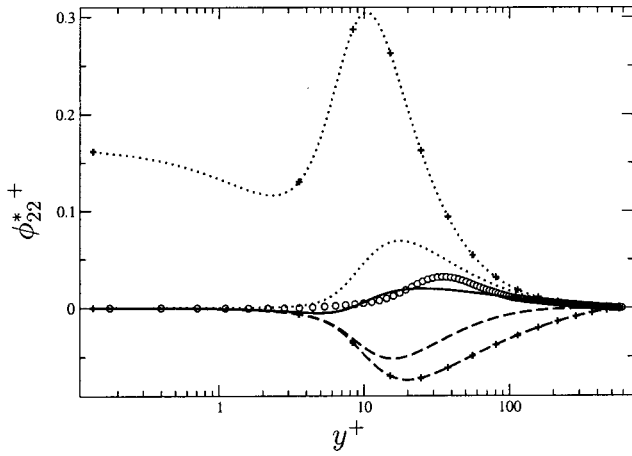
FIG. 6. Elliptic blending model: different contributions to \phi_{22}^* . +\cdots+\phi_{22}^h (SSG model); \cdots k\alpha\phi_{22}^h ; +---+\phi_{22}^w ; ---(1-k\alpha)\phi_{22}^w ; ---\phi_{22}^*=(1-k\alpha)\phi_{22}^w+k\alpha\phi_{22}^h ; \circ\phi_{22}^* from the DNS.
