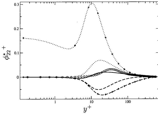
FIG. 6. Elliptic blending model: different contributions to \phi_{22}^* . +\cdots+\phi_{22}^h (SSG model); \cdots k\alpha\phi_{22}^h ; +---+\phi_{22}^w ; ---(1-k\alpha)\phi_{22}^w ; ---\phi_{22}^*=(1-k\alpha)\phi_{22}^w+k\alpha\phi_{22}^h ; \circ\phi_{22}^* from the DNS.
