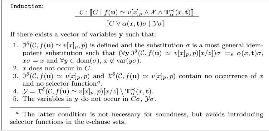
Fig. 2: The Induction rule
