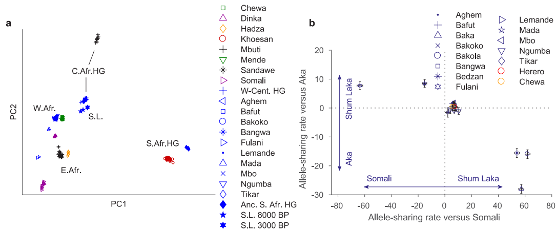
Extended Data Fig. 3 | Alternative PCA and allele-sharing analyses. a , Broad-scale PCA (differing from Fig. 2a by projecting all present-day Cameroon populations; again using 593,124 Human Origins SNPs). Groups shown in blue were projected onto axes computed using the other populations. HG, hunter-gatherers. The grouping marked W-Cent. HG consists of Aka and Cameroon hunter-gatherers (Baka, Bakola and Bedzan). The majority of the present-day Cameroon individuals fall in a tight cluster near other West Africans and Bantu-speakers. b , Relative allele sharing (mean \pm s.e., multiplied by 10,000, computed on 538,133 SNPs, as in Fig. 3b) with the Shum Laka individuals versus
