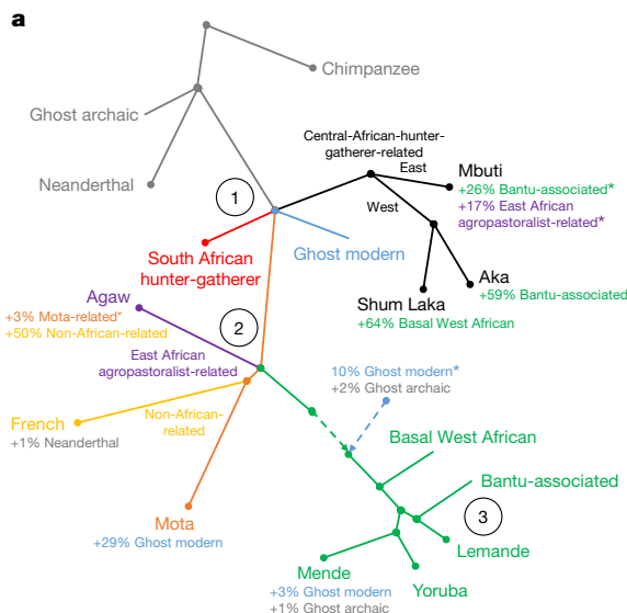
Fig. 4 | Admixture graph results. Points at which multiple lineages are shown diverging simultaneously indicate splits occurring in short succession (the order of which we cannot confidently assess) but do not represent exact multifurcations. Key points are (1) the early modern human split, (2) East African divergences and (3) the expansion of ancestry associated with Bantu-speakers. Branch lengths are not drawn to scale. a , Full model (Extended Data
