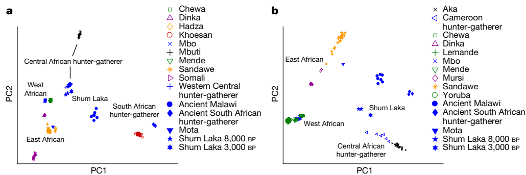
Fig. 2 | PCA results. a , Broad-scale analysis. b , Narrow-scale analysis. Groups in blue (including ancient individuals (filled symbols)) were projected onto axes computed using the other populations, using 593,124 SNPs (Methods). The
