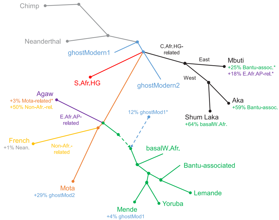
Extended Data Fig. 7 | Schematic of the second alternative admixture graph. Results are shown with a single-component deep source for West Africans. Branch lengths are not drawn to scale. Points at which multiple lineages are shown diverging simultaneously indicate splits that occur in short succession (the order of which we cannot confidently assess) but are not meant to
