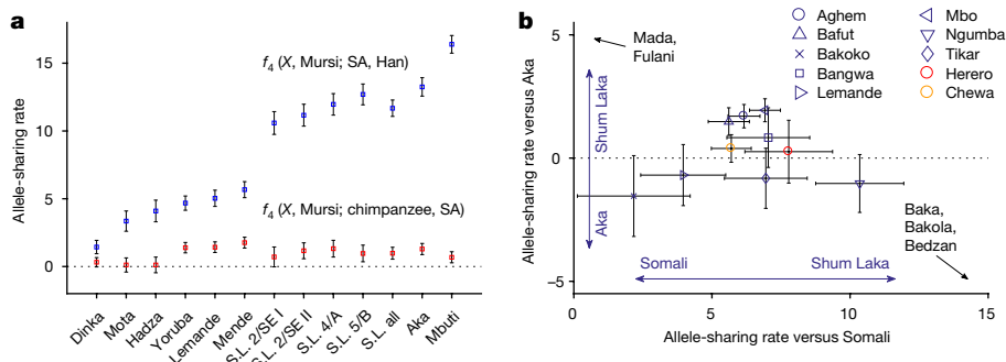
Fig. 3 | Allele-sharing statistics. a , Statistics sensitive to deep ancestry (mean \pm 2 s.e., multiplied by 1,000). Blue, deeper than non-Africans; red, deeper than southern African hunter-gatherers; computed on 1,121,119 SNPs. SA, ancient South African hunter-gatherers; S.L., Shum Laka. b , Relative allele sharing (mean \pm s.e., multiplied by 10,000; computed on 538,133 SNPs) with the
