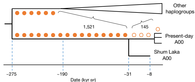
Fig. 1 | Y chromosome phylogeny. Circles represent mutations along the (unrooted) A00 lineage where we observe the alternative (filled) or reference (empty) allele in the A00 sequence carried by Shum Laka individual 2/SE II, kyr, thousand years.
