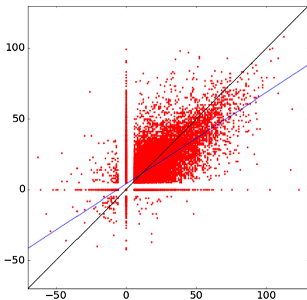
Figure 2.3.2. BLT comparisons between ARMOR3D weekly (product 2.3.1) and in situ: scatterplot diagram between Argo profiles in situ BLT in the Tropical Pacific (15°N-15°S,130°E-80°W) (abscissa), and the corresponding collocated BLT from ARMOR3D (ordinate); units are metres. The black line along the diagonal corresponds to the perfect fit; the flatter blue line corresponds to the linear regression between ARMOR3D and in situ data.
