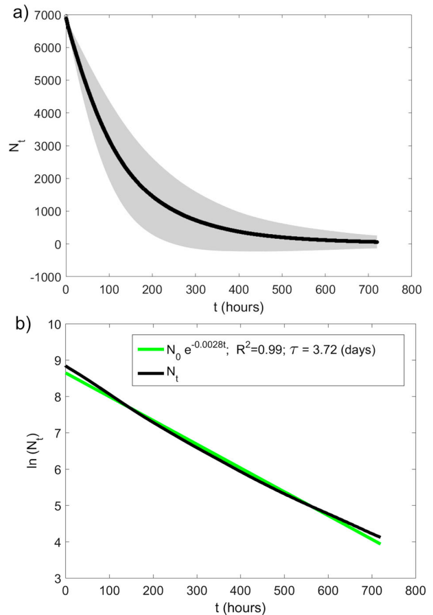
Figure 2.8.2. (a) Time evolution of the number of particles inside the area (HF radar coverage for the Ibiza Channel domain) as a function of time, averaged over 5000 initializations. (b) Result of the exponential fit (green curve) to the averaged curve (in black) shown in (a). In (b) \ln(N_t) is displayed on the y-axis.
