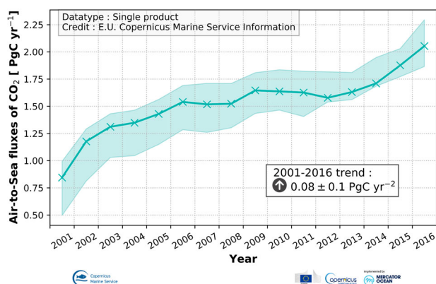
Figure 2.10.2. Global integrated yearly ocean uptake of CO 2 derived from the Ocean Monitoring Indicator (OMI) 'Global Surface Ocean CO 2 flux' (Product 2.10.2a). Plain line, best model after Denvil-Sommer et al. (2019); range, empirical 95% confidence interval computed from 25 samples.
