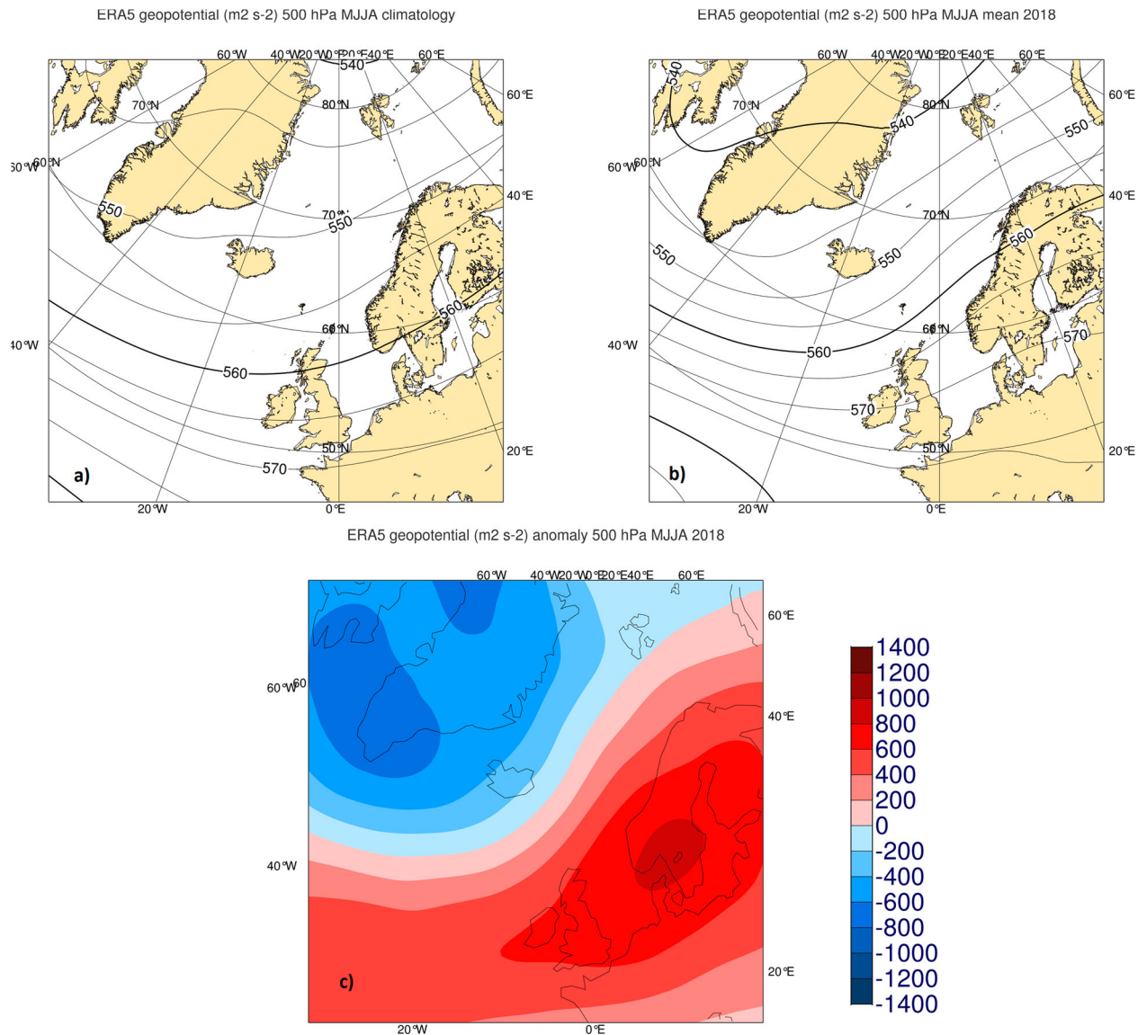
Figure 4.4.3. May-August mean circulation at 500 hPa in 2018: (a) geopotential height climatology; (b) geopotential height in 2018 and (c) geopotential anomaly ( \text{m}^2 \text{s}^{-2} ) relative to 1981–2010 climatology. The results are generated from product ref. 4.4.2.
